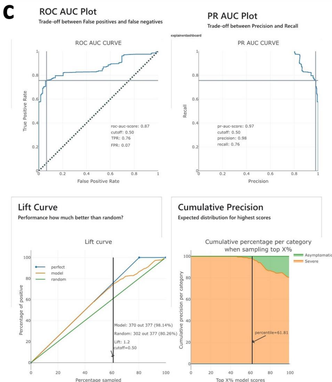
Figure 5(c): ExplainerDashboard displayed Classification Stats
