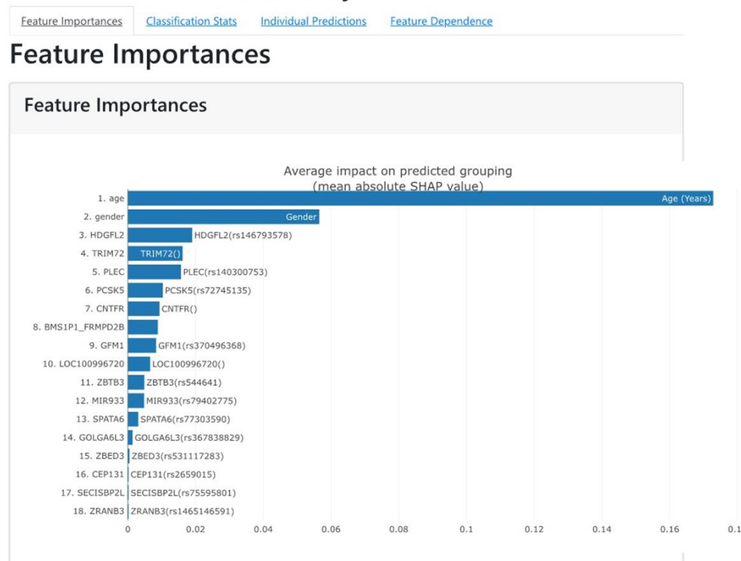
Figure 5(a): ExplainerDashboard displayed SHAP feature importance plot.
