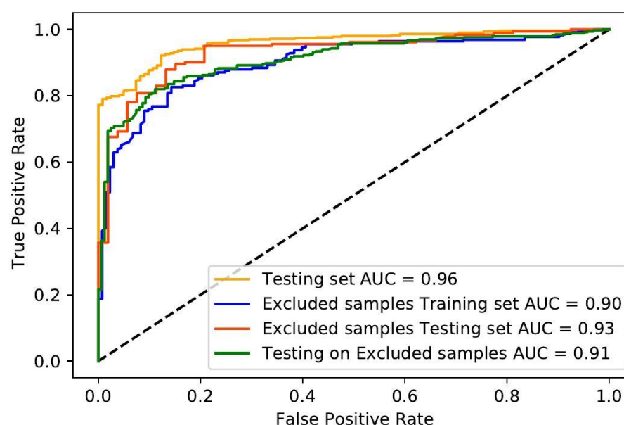
Figure 4: HGSP model performance considering out-of-sample model validation in all case studies.
