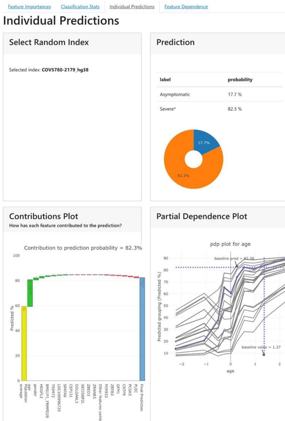
Figure 5(d): ExplainerDashboard Individual predictions plot
