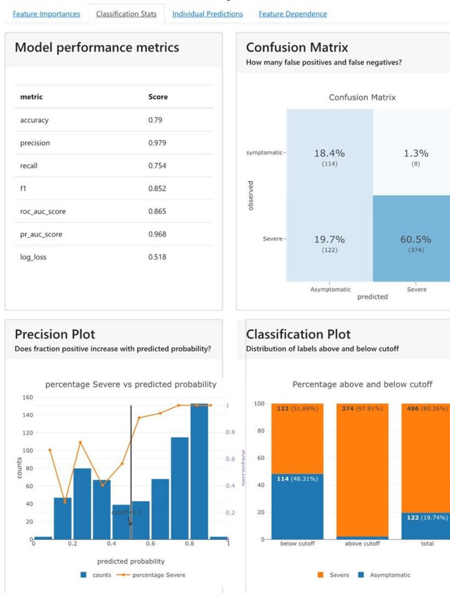
Figure 5(b): ExplainerDashboard displayed Classification Stats.
