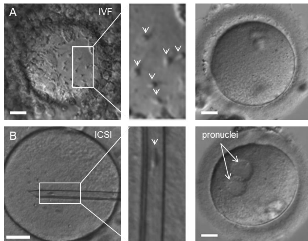
Figure 3: Microscopic documentation of medically-assisted reproduction with CATSPER2 -/- sperm. (A) Left: Representative micrograph of an oocyte with CATSPER2 -/- sperm from patient C5 attached to the zona pellucida (indicated by arrows in the zoomed-in image, middle ), taken after overnight incubation of sperm and oocyte for in-vitro fertilization (IVF). None of the five oocytes subjected to IVF was fertilized ( right , representative example). (B) Left: Representative micrograph of an oocyte with an inserted glass pipette containing a CATSPER2 -/- sperm cell from patient C5 (indicated in the zoomed-in image, middle ) for intracytoplasmic sperm injection (ICSI). Nine out of the 15 eggs injected with CATSPER2 -/- sperm developed two pronuclei ( right , representative example) indicating fertilization. Scale bars represent 30 \mu m.
