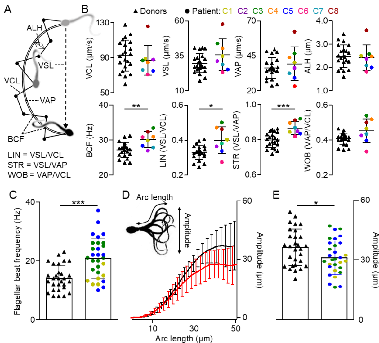
Figure 4: Analysis of basal motility and flagellar beat of control and CATSPER2 -/- sperm. (A) Illustration of the swimming path and kinematic parameters of a sperm cell determined by computer-assisted sperm analysis (CASA). Curvilinear velocity (VCL) represents the frame-to-frame track of the sperm head, from which the average-path velocity (VAP) is calculated. The beat-cross frequency (BCF) is the frequency at which the sperm track crosses the VAP path. The amplitude of lateral head displacement (ALH) is the average deviation of the head from the VAP path. The straight-line velocity (VSL) is derived by charting a direct path between the first and last head position in the image sequence. The linearity (LIN), straightness (STR), and wobble (WOB) are indicators for the linearity of the path trajectory. (B) Scatter plots (mean \pm SD) of kinematic parameters of control (black triangles, n = 22 ) and CATSPER2 -/- sperm from patients C1-C8 (color-coded circles). (C) Scatter plots (mean \pm SD) of the flagellar beat frequency of single head-tethered control sperm from donors (black triangles, n = 29 from six experiments) and of sperm from CATSPER2 -/- patients (color-coded circles, n = 30 from three experiments). (D) Maximal beat amplitude (mean \pm SD) along the arc length of the flagellum of the head-tethered control (black) and CATSPER2 -/- (red) sperm analyzed in (C). (E) Scatter plots (mean \pm SD) of the maximal beat amplitude of the control (black triangles) and CATSPER2 -/- (color-coded circles) sperm reported on in (C) and (D). *P < 0.05, **P < 0.01, ***P < 0.001, unpaired t-test with Welch's correction.
