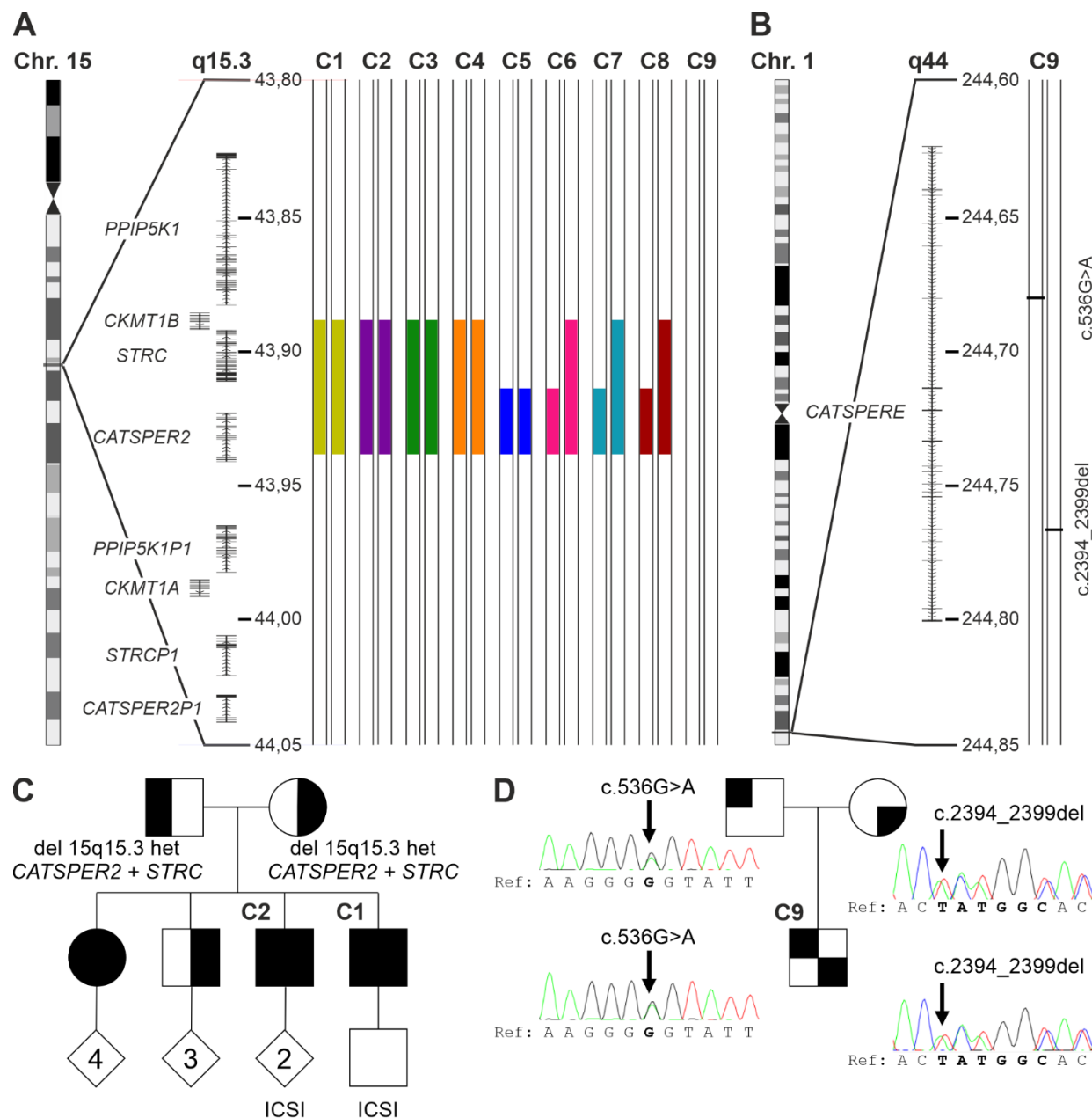
Figure 2: Genetic aberrations identified in CatSper-deficient patients. (A) Schematic depiction of chromosome 15, magnified region q15.3 including genes, and the identified deletions (represented as filled color-coded bars) in patients C1-C8, but not patient C9. All positions according to hg19/GRCh37. (B) Schematic depiction of chromosome 1, magnified region q44 and compound-heterozygous variants (see panel D) (c.536G>A and c.2394_2399del) of CATSPERE (NM_001130957.2) identified in patient C9. (C) Family pedigree of patients C1 and C2, who are brothers. Their sister is also homozygous for the deletion at 15q15.3, whereas their mother, father, and third brother are heterozygous carriers. (D) Family pedigree of patient C9, demonstrating that the father and mother are carriers of the missense variant (c.536G>A) and in-frame deletion (c.2394_2399del), respectively. Of note, in Schiffer et al. (2020), we already showed array-CGH data from patients C1-C5, reporting on the deletion of CATSPER2 in these five patients for the first time.
