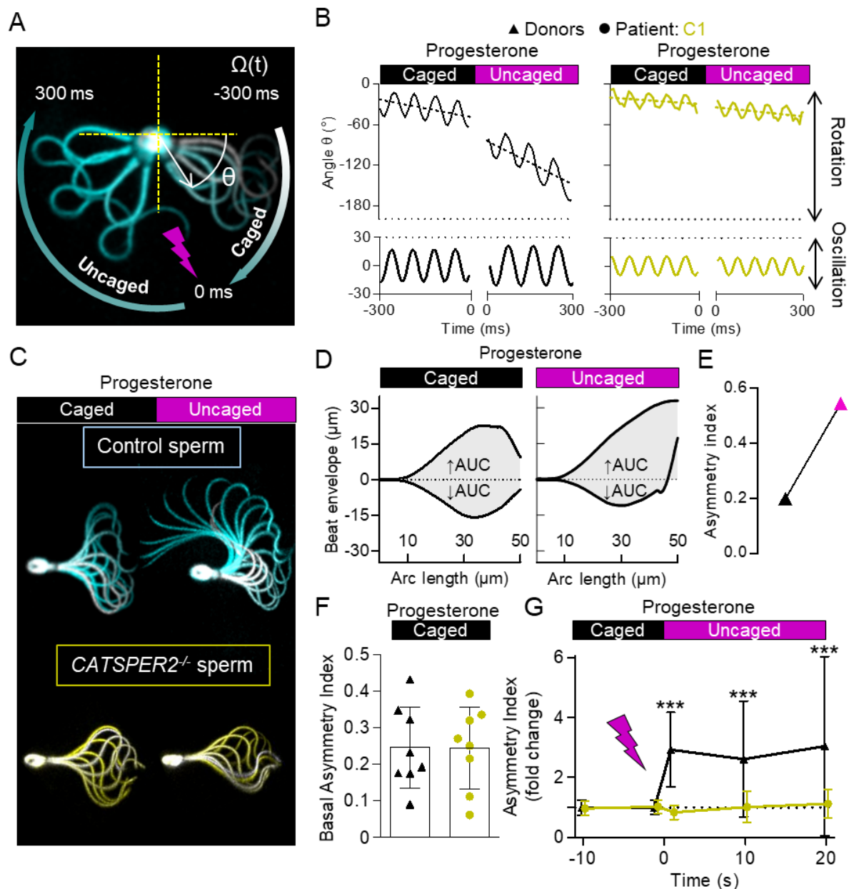
Figure 6: Progesterone-induced changes in flagellar beat of control and CATSPER2^{-/-} sperm. (A) Representative time-lapse overlays of three beat cycles before and after uncaging progesterone (2 \mu M ) of a pivoting head-tethered capacitated control sperm from a donor. (B) Change of angle \theta over time (solid line, upper panels) with the corresponding slope (dotted line) and fitted sine wave of the oscillation (lower panels) of control (black, left panel) and CATSPER2^{-/-} (gold, right panel) sperm from patient C1 before and after uncaging progesterone. The corresponding frequency and amplitude of the flagellar beat were derived from the fitted sine wave and the rotation velocity, \Omega(^{\circ}\cdot s^{-1}) was derived by the slope of the change of \theta over time. (C) Representative overlays of a single beat cycle of a control (cyan) and a CATSPER2^{-/-} (gold) sperm before and after the uncaging of progesterone (2 \mu M ). (D) The area under the curve outlined by the beat envelope above ( \uparrow AUC ) and below ( \downarrow AUC ) the head-midpiece axis of a control sperm
