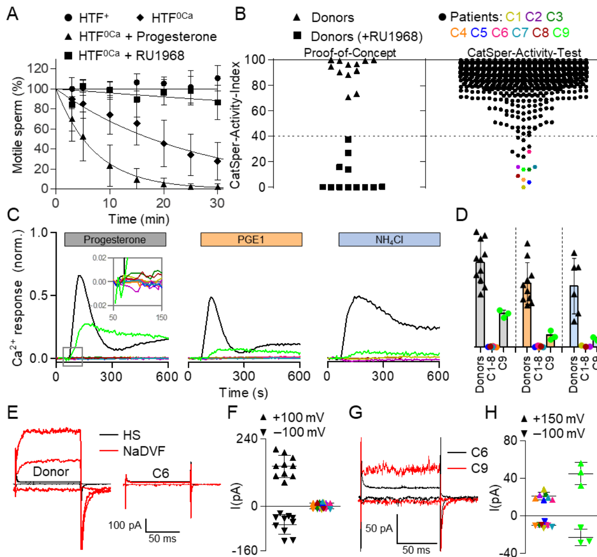
Figure 1: Identification of patients with loss or impaired CatSper function. (A) Changes in the fraction of motile sperm (mean \pm SD) upon dilution of semen samples from donors in Ca 2+ -free HTF (HTF 0Ca ) (diamonds), HTF 0Ca containing progesterone (10 \mu M) (triangles), or HTF 0Ca containing the CatSper-inhibitor RU1968 (15 \mu M) (squares), relative to the fraction of motile sperm determined upon dilution of the respective semen sample in control HTF + (circles) at t = 0 (set to 100%). An exponential decay curve was fitted to the change in the fraction of motile cells averaged over all replicates. (B) Left: CatSper-Activity-Indices (CAI, see explanation in the text) determined 15 minutes after dilution of semen samples from donors in HTF + (Buffer A) and HTF 0Ca containing progesterone (triangles) (Buffer B) or Buffer B also containing RU1968 (15 \mu M) (squares). Right: CAI values from semen samples of men undergoing semen analysis (n = 2,286); see explanation in the text as to the dotted line. Patients with confirmed loss or impaired CatSper function are labeled C1-C9 and indicated with a color-coded circle. (C) Representative Ca 2+ signals in sperm from patient C1-C9 (color coded) and a donor (black) evoked by progesterone (3 \mu M), PGE1 (3 \mu M), or NH 4 Cl (30 mM) relative to the maximal signal amplitude evoked by ionomycin (3 \mu M)
