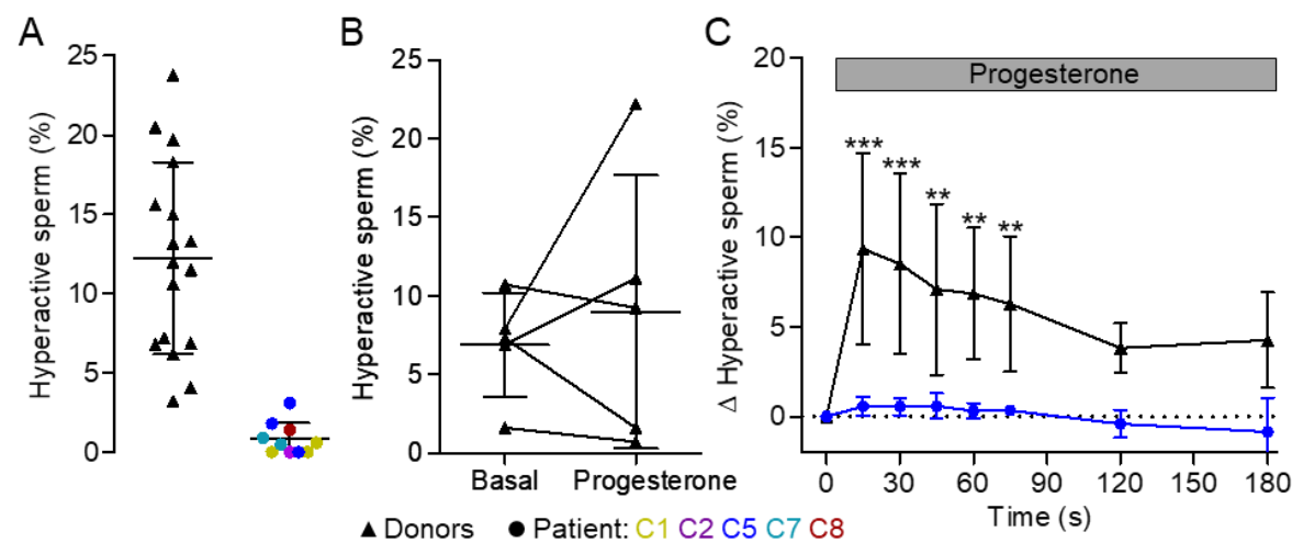
Figure 5: Capacitation- and progesterone-induced hyperactivation of control and CATSPER2 -/- sperm. (A) Scatter plot (mean \pm SD) of the fraction of hyperactivated control (black triangles, n = 17) and CATSPER2 -/- sperm (color-coded circles, n = 10 experiments with sperm from patients C1, C2, C5, C7, and C8) upon incubation under capacitating conditions. (B) Paired plots of the fraction of hyperactivated control sperm from donors before (basal) and after treatment (5 min) with progesterone (5 \mu M) determined by standard CASA. (C) Change of the fraction (mean \pm SD) of hyperactivated control sperm from donors (black, n = 5) and from a CATSPER2 -/- patient (blue, n = 3, i.e., three independent experiments with sperm from patient C5) evoked by mixing with progesterone (gray bar), corrected for the fraction of hyperactivated sperm determined after mixing with HTF ++ alone (set to 0 at t = 0 s), and determined by a custom kinetic CASA technique. Experiments were performed with sperm incubated under capacitating conditions. **P < 0.01, ***P < 0.001, ANOVA with Dunnett's multiple comparison test versus the respective controls (t = 0 s).
