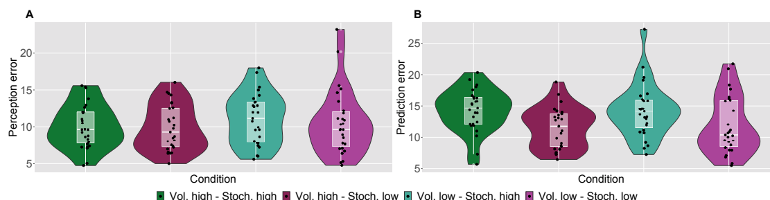
Figure 2. Participant’s model-naïve performance in the task. Violin plots of participant Root Mean Square Error (RMSE) for each condition for A : rating and B : prediction responses as compared with the input.
