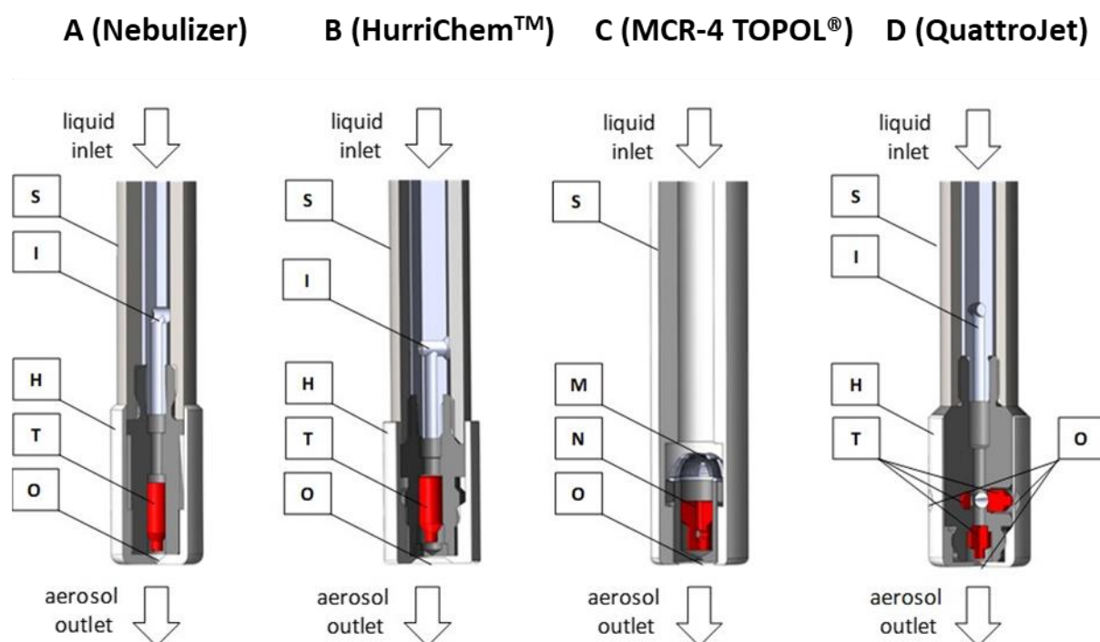
Figure 1: 90° sectional views of the head regions of the nozzles. Legend: O = outlet orifice; H = nozzle head; I = bar inlay with distal transverse borehole; M = double metal grid; N = fixed needle; S = shaft; T = twist body.
