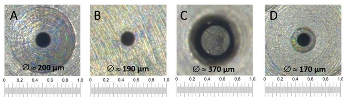
Figure 2: Light microscopic images of the outlet orifices with determined orifice diameters of the examined nozzles; scaling in mm. Nozzles A, B, C, D
