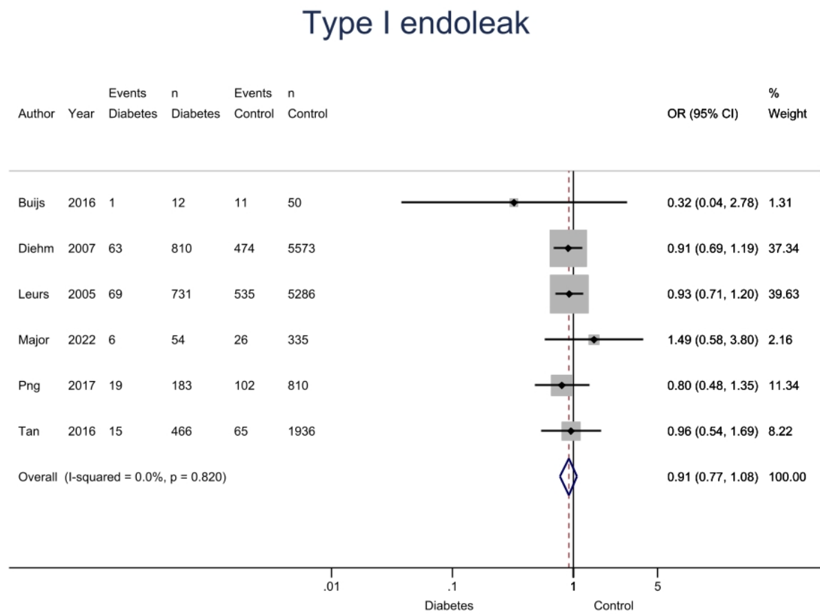
Figure 3 – Forest Plot of Type I Endoleak post EVAR in those with DM and controls.
