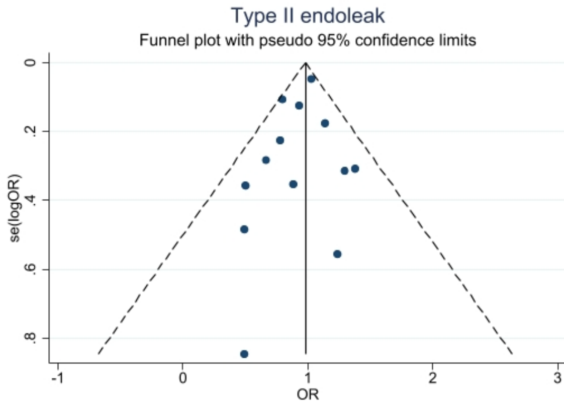
Figure 12 – Funnel plot of type II endoleak
