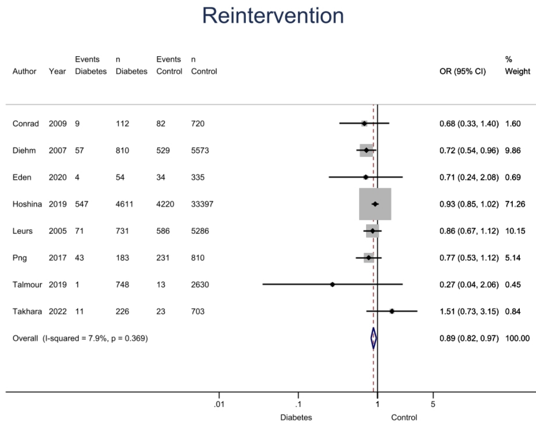
Figure 2 - Forest Plot of reintervention rates post EVAR in those with DM and controls.
