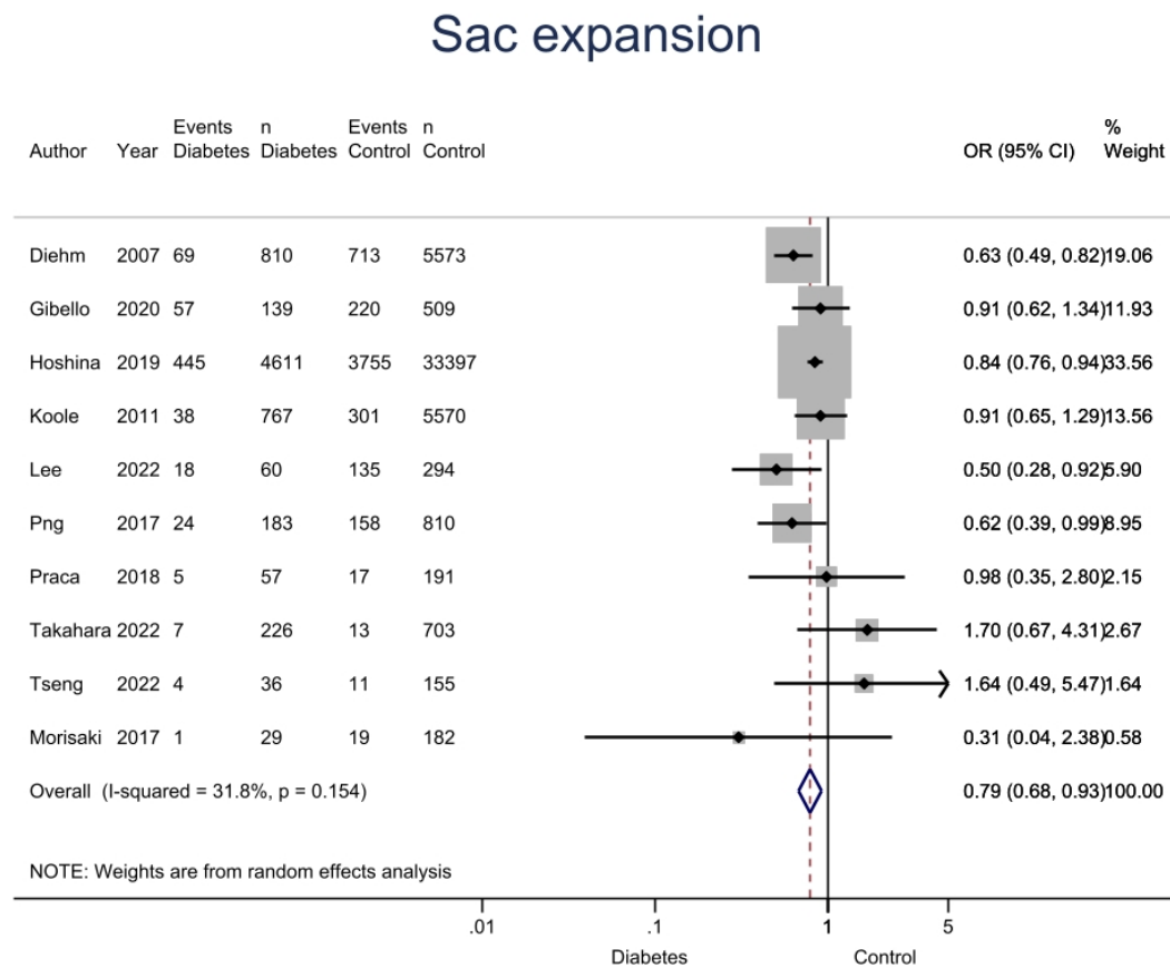
Figure 6 – Forest plot of AAA Sac expansion in those with DM and controls
