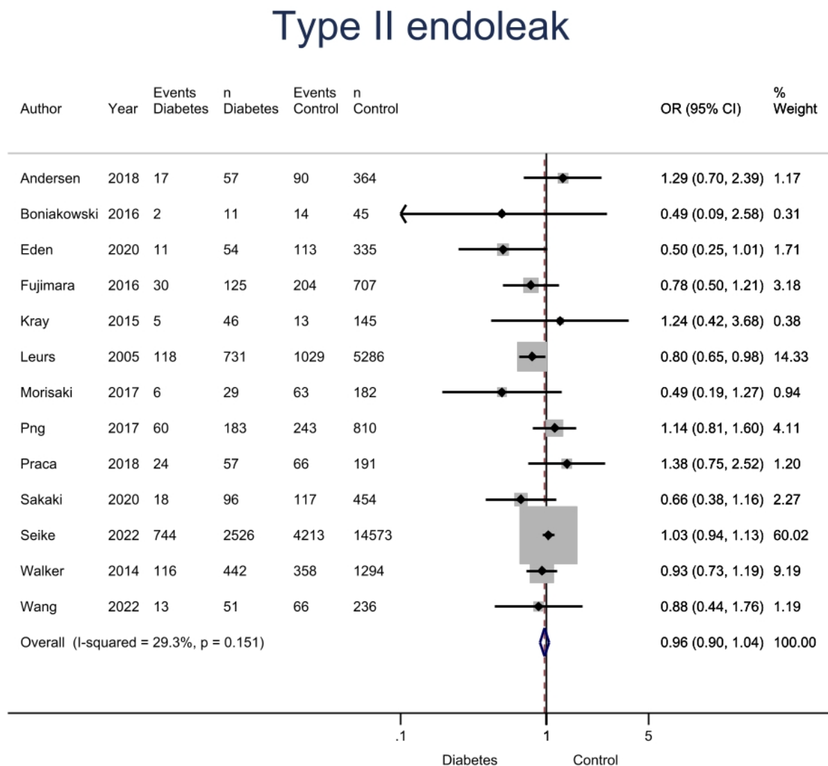
Figure 4 - Forest Plot of Type II Endoleak post EVAR in those with DM and controls.
