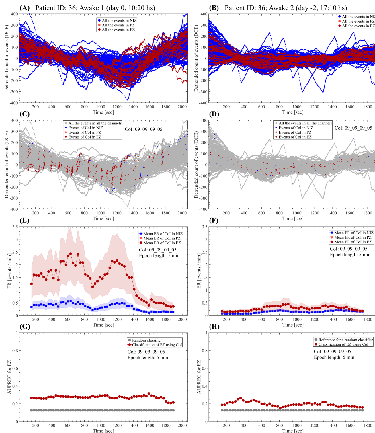
Figure S22: Comparing the fast-ultradian dynamics between two SEEG recording sessions in awake state. (A, B) Detrended cumulative count of events (cumulative residual) including all events subtypes (epileptic and non-epileptic) detected by the NODE algorithm (80 clusters). (C, D) Cumulative residual showing all the detected events (gray dots) and the discharges pertaining to the cluster 09_09_09_05 in color (NIZ: blue dots, PZ: light red dots, EZ: dark red dots). (E, F) Mean rate of events pertaining to the cluster 09_09_09_05. The dots correspond to the mean value of the
