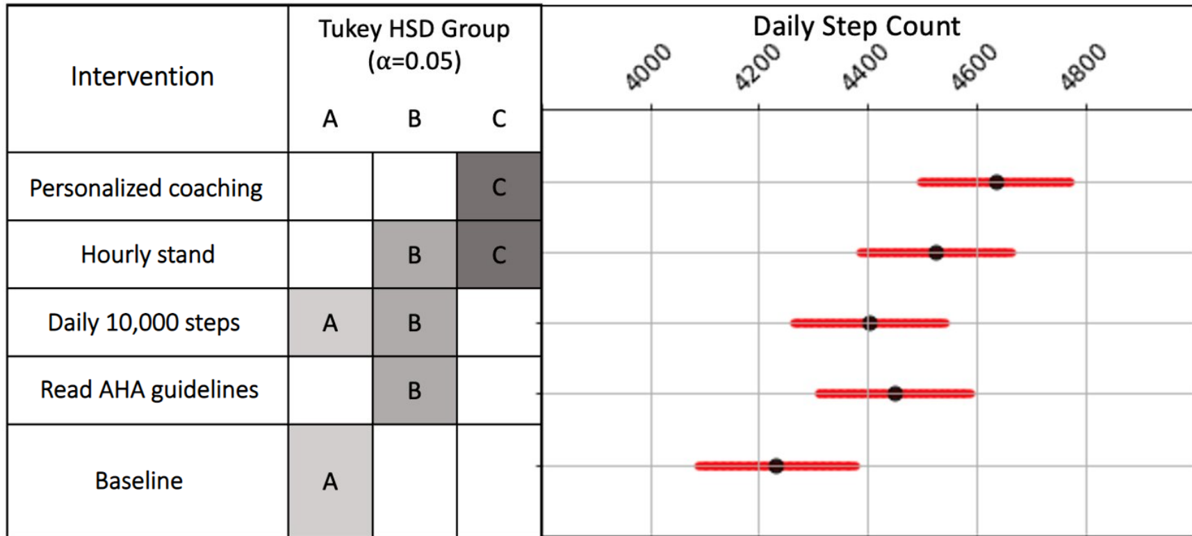
Figure 2. Mean daily step count for the 1-week baseline period and for the four interventions in the modified intention-to-treat subset of the randomized crossover MyHeart Counts Study. Mean daily step count was recorded by the MyHeart Counts iPhone app. Error bars show 95% CI. Interventions assigned to different Tukey groups are significantly different from each other.
