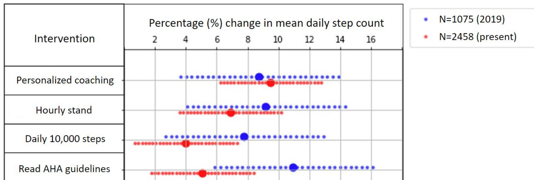
Figure 3. Comparison of intervention effects in present data (N=2458) as compared to previously published data (N=1075) in the modified intention-to-treat subset of the MyHeart Counts randomized crossover trial. Error bars show 95% CI.
