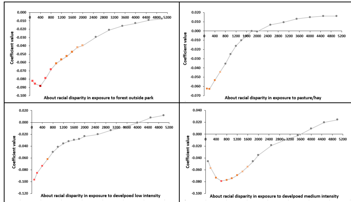
Figure 8. Coefficient values describing the associations between racial disparity in landscape and urban exposure within multiple buffer distances (100m-5km) and racial disparity in SARS-CoV-2 infection rates. Coefficient values are represented as dots with different colors. The gray color indicates nonsignificant associations, p \geq 0.1 . Strong to light red colors indicate significant associations at different levels, p < 0.001 , p < 0.01 , p < 0.05 , and p < 0.1 (see detailed numbers in Table 3).
