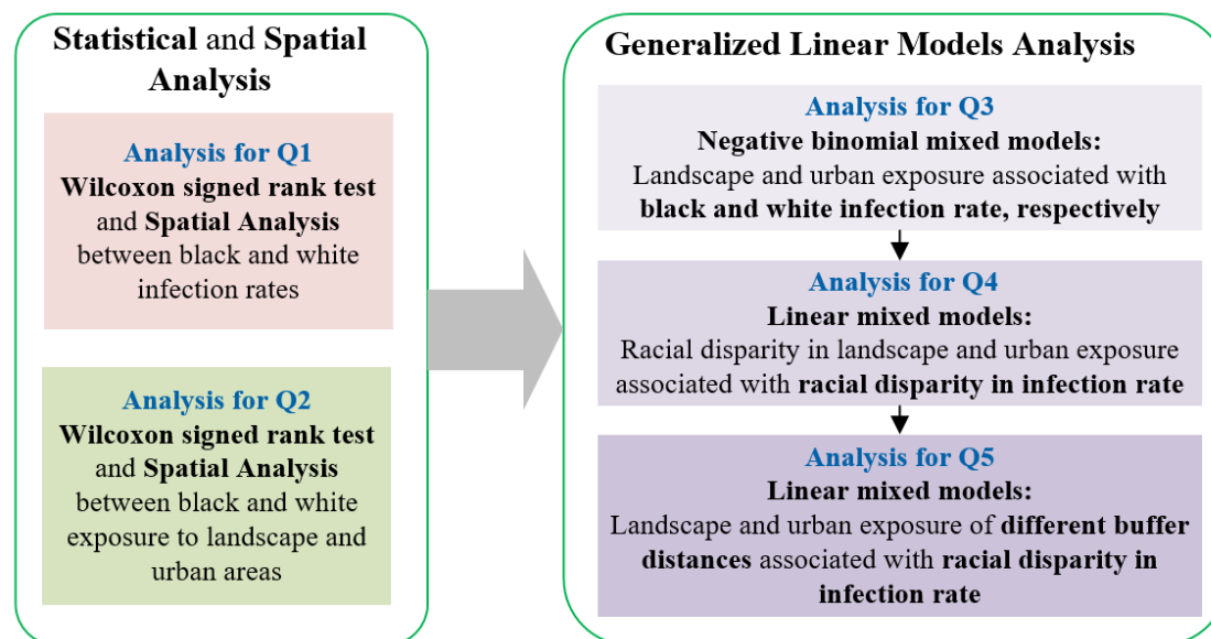
Figure 2. The framework of statistical analysis includes five components. Each component aimed to answer one of five proposed research questions.
