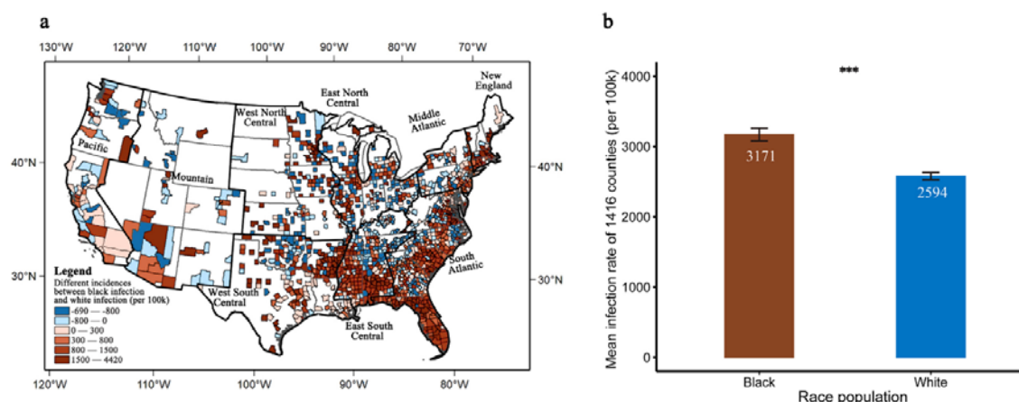
Figure 3. Difference in SARS-CoV-2 infection rates between black and white people.
