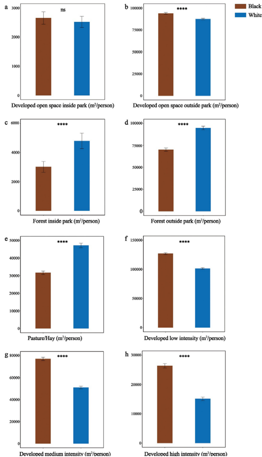
Figure 4. Comparisons of landscape and urban exposure between black and white people (within the 400 m buffer distance). A Wilcoxon two-sample test was used to compare eight types of landscape and urban exposure. The histogram shows mean values of exposure for black and white people in 1416 counties. The error bar represents standard error of the mean. '****' p < 0.0001 , 'ns' p \geq 0.1 .
