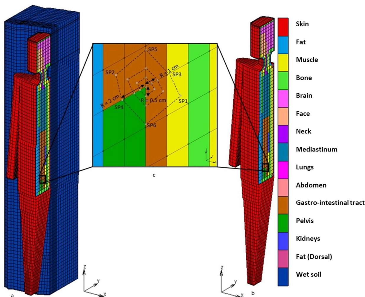
Fig. 2 a: Coarse model lying on a support structure (CMS), Fig. 2 b: Coarse model without support structure (CM), Fig. 2 c: Detailed view of measurement points C, SP 1 , ..., SP 6 along different radii R = 0.5 cm, 1 cm, 2 cm. For the octahedra see Fig.4. Only the contour lines of the octahedra are shown for clarity.
