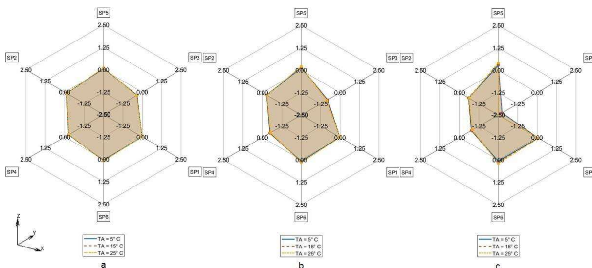
Fig. 9: Difference in TDE deviation in D_{MAX} between CM vs CTM for T_A = 5^\circ \text{C} (Solid line), T_A = 15^\circ \text{C} (Dashed line), T_A = 25^\circ \text{C} (Dash-dotted line) a. R = 0.5 \text{ cm} , b. R = 1 \text{ cm} , c. R = 2 \text{ cm}
