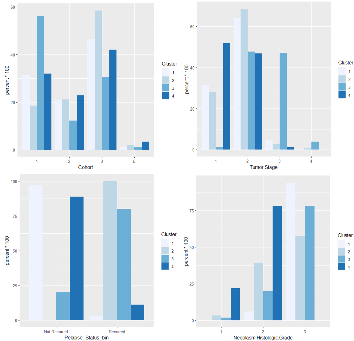
Picture 4 Categorical subgroup frequency group by 4 clusters
