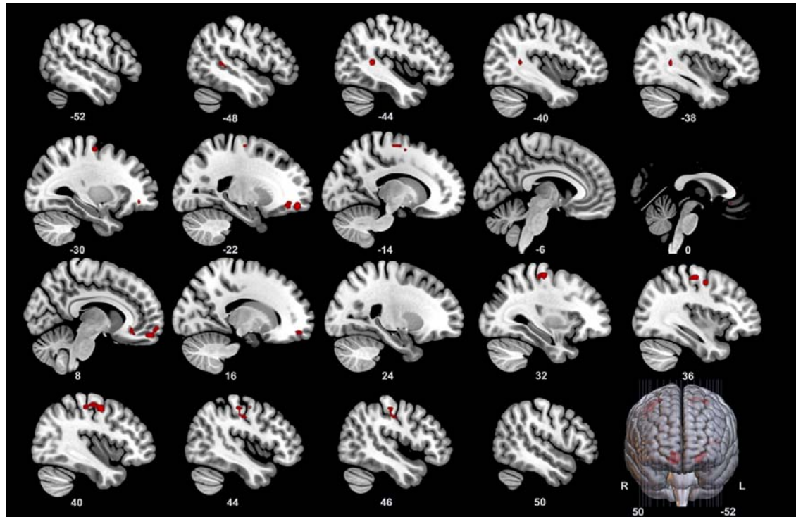
Figure 4. The results of paired two sample t-test of the ALFF values from the resting-state functional MRI data of the patients before and after the surgery. The results are shown as the t-value of each voxel in the figures ( P < 0.05 , multi-comparison correction through false discovery rate). The voxels in red indicated significantly higher local activations after the surgery comparing to the data before the surgery in an average level. ALFF: amplitude of low-frequency fluctuation.
