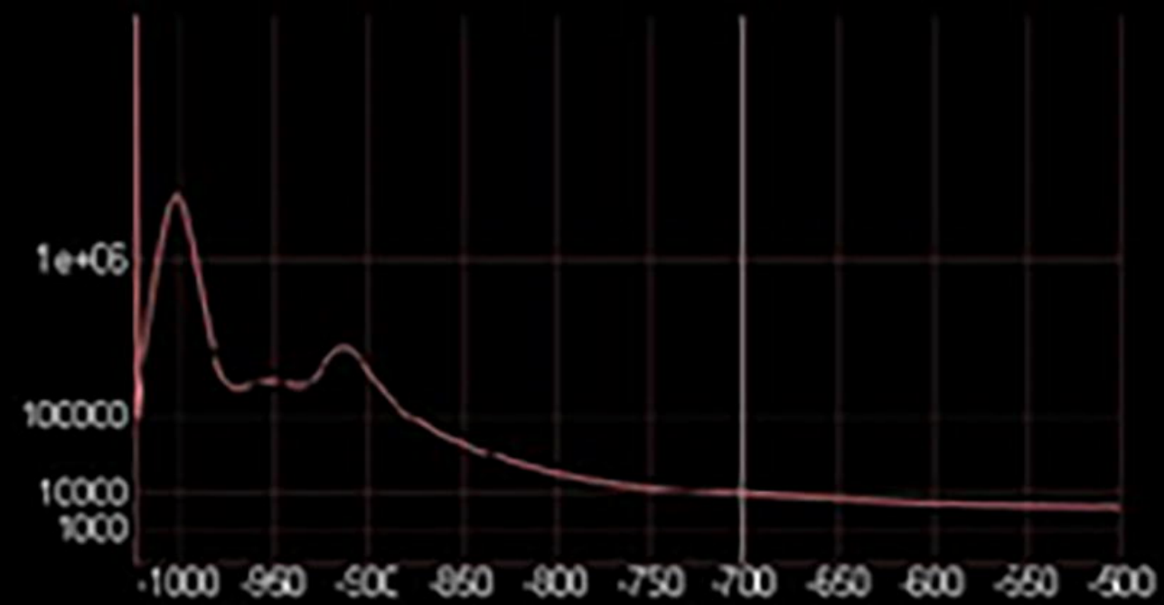
Histogram
