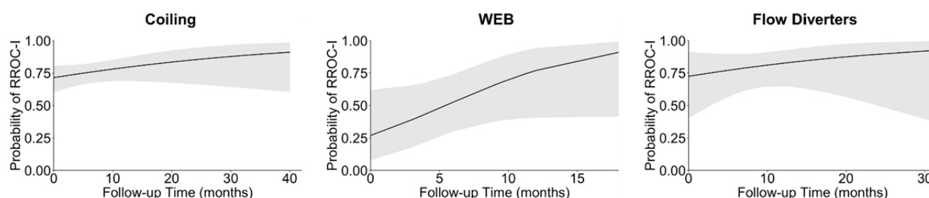
Figure 2. LGLMM model fits for probability of RROC-I as a function of follow-up time for the evaluated endovascular therapy techniques. Grey shading represents CI 95%.
