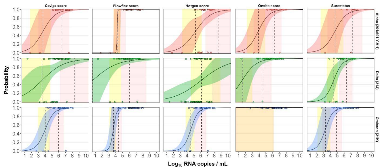
Figure 3: Limit of detection analyses of upper-respiratory samples positive by RT-qPCR for five SARS-CoV-2 Ag-RDT tests (Covios, Hotgen, Onsite, Flowflex and SureStatus) using NP swabs. The log 10 RNA copies on the x axis were plotted against a positive (1.0) or negative (0.0) Ag-RDT result on the y axis. Fill curves show logistic regressions of the viral load on the Ag-RDT result; vertical dashed lines indicate log 10 RNA copies subjected to the test at which 50% and 95% LOD of the samples are expected positive based on the regression results. No significant differences were observed.
