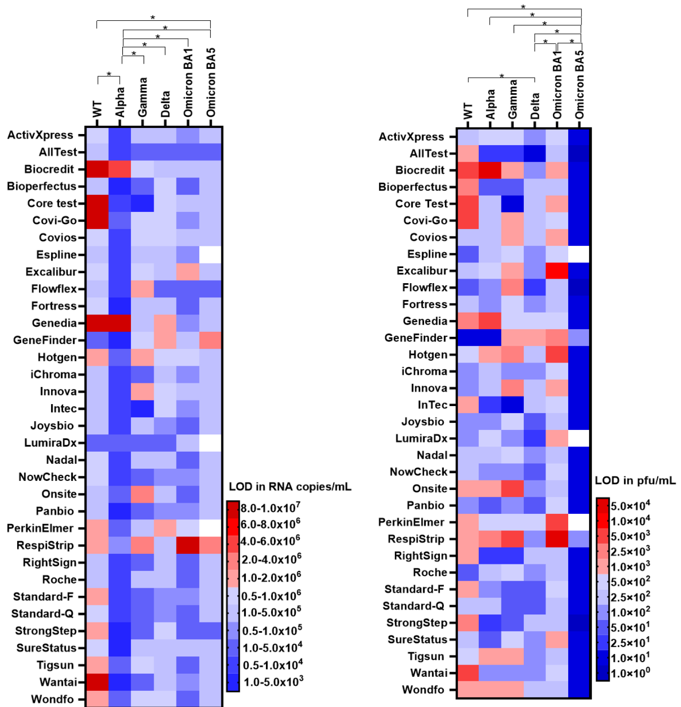
Figure 1. Heatmap comparing the LODs of 34 Ag-RDT using the Ancestral (WT), Alpha (B.1.1.7), Gamma (P.1), Delta (B.1.617.2) Omicron (BA.1) and Omicron (BA.5) variants on pfu/mL (A) and RNA copies/mL (B). Data of the Ancestral, Alpha and Gamma have been taken from our previously published work (21). Blue colours indicate LODs fulfilling the DHSC (for pfu/mL) and WHO criteria (for RNA copies/mL). * = p \leq 0.05 between VOCs.
