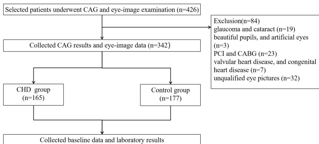
Figure 2 Study flowchart
