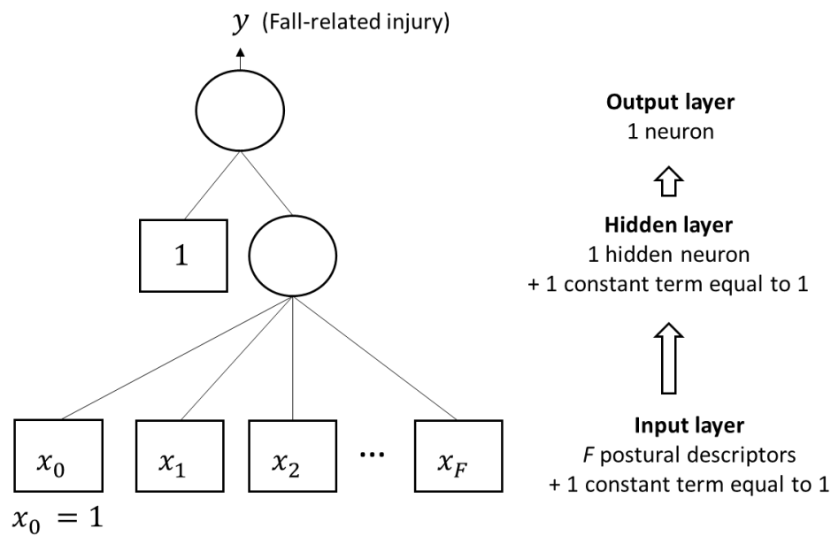
Figure S2.. Graphical representation of the neural network model. Information propagates from the bottom (input) to the top (output) layer, via a single intermediate (hidden) layer that includes a single neuron. In our study, input variables were the postural descriptors ( x_j j=1, \dots, F ) and a constant x_0 equal to 1, and the output variable y was the probability of belonging to the class Injured due to a fall .
