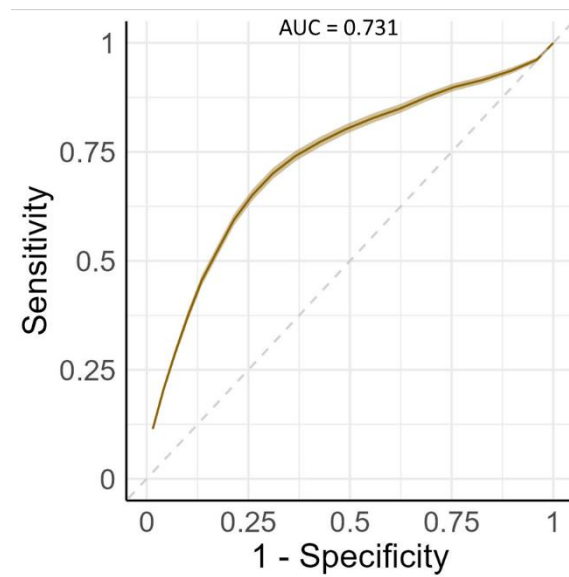
Figure 2. Receiver Operating Characteristic (ROC) curves for the Neural Network model for prediction of the fall-related injury event during the selection course from the selected postural predictors. Error bars of the ROC curves indicate 95% confidence interval for the area under the ROC curve (AUC).
