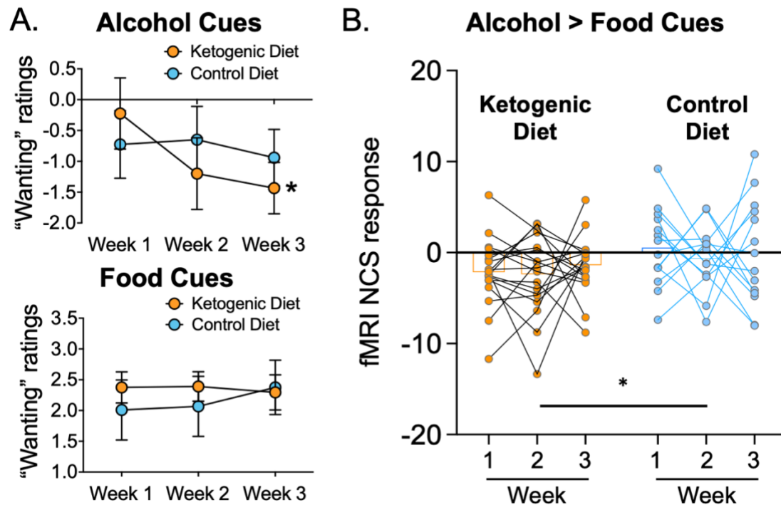
Figure 2. A) Alcohol “wanting” ratings of alcohol cues were lower in KD than Control diet after diet initiation. There were no group differences for “wanting” ratings caused by food-cues. B) The fMRI NCS response was lower in the KD group than the Control Diet throughout the 3 weeks of dietary intervention.
