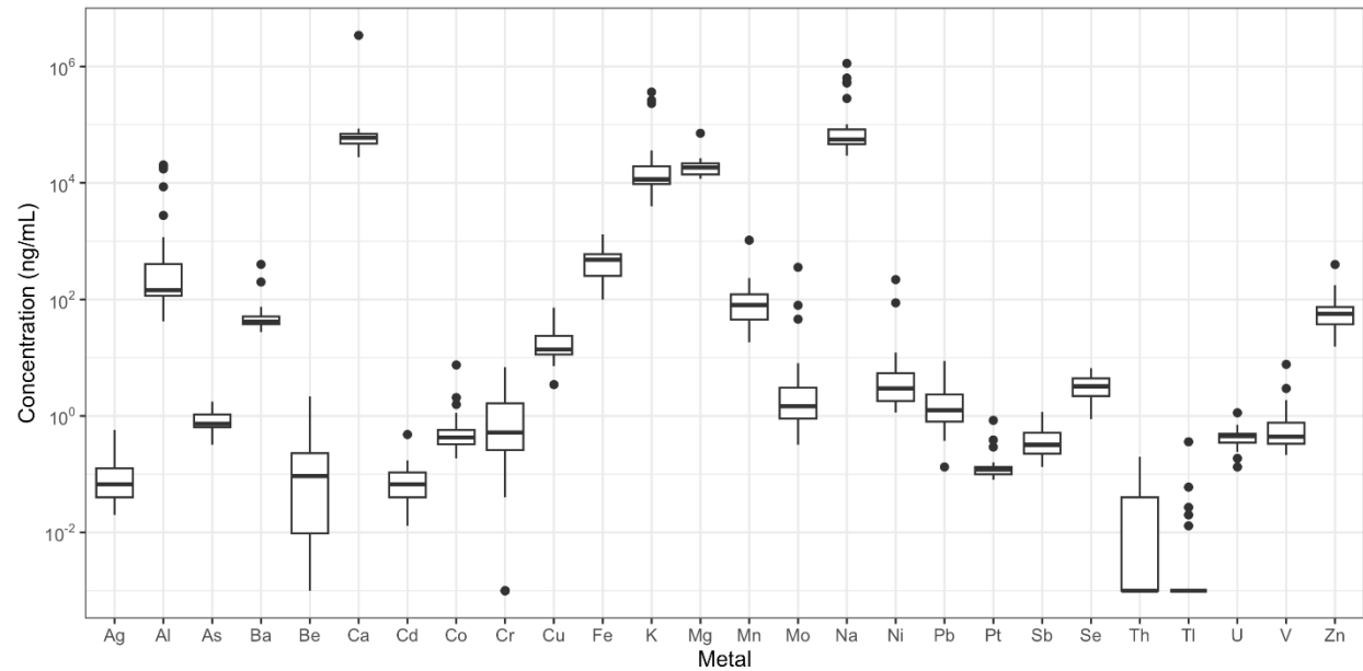
Fig. 3. Metal concentration variability for studied sewersheds (N=26), Jefferson County, Kentucky (USA). Metal concentrations are plotted as log concentrations. The box regions represent the first to third quartile, and the black dots represent the outliers. Data were transformed by adding 0.001 to values of 0 or not detected for data distributions.
