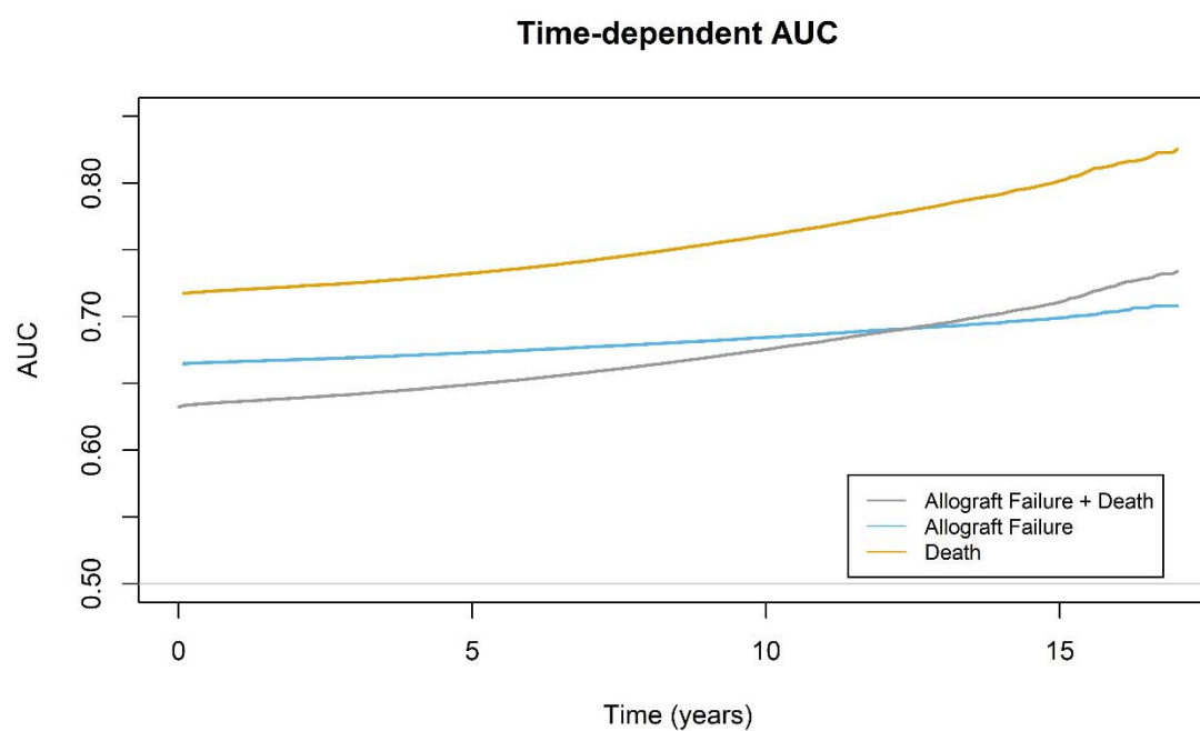
Figure 6. Time-dependent AUC
