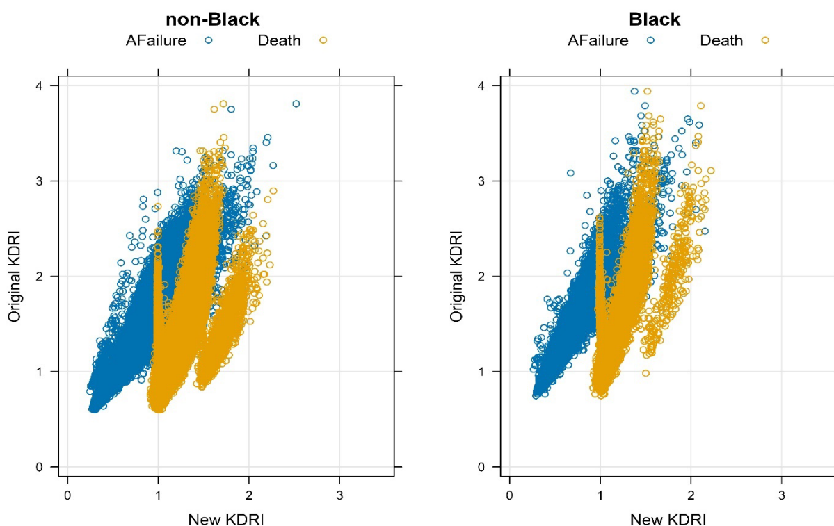
Figure 3. KDRI comparison
