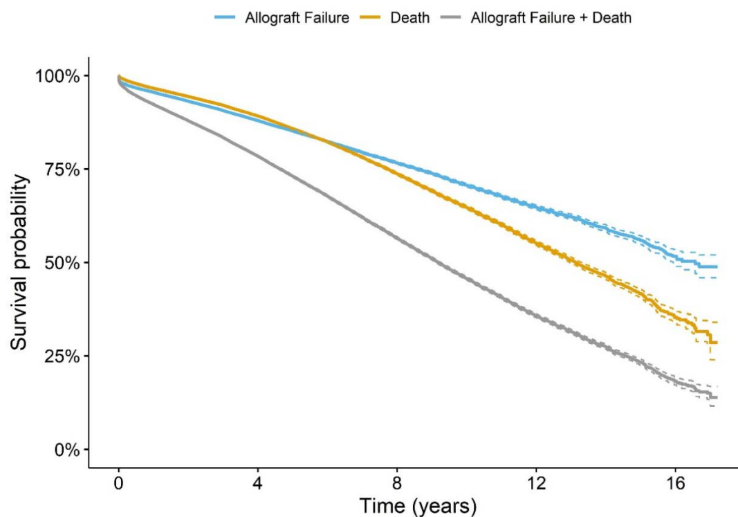
Figure 5. Kaplan-Meier estimates
