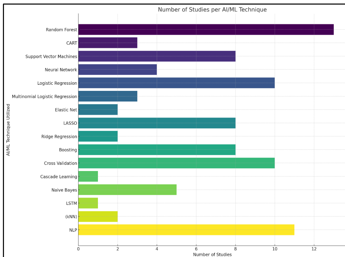
Figure 4: Overall counts of AI/ML algorithms employed.
