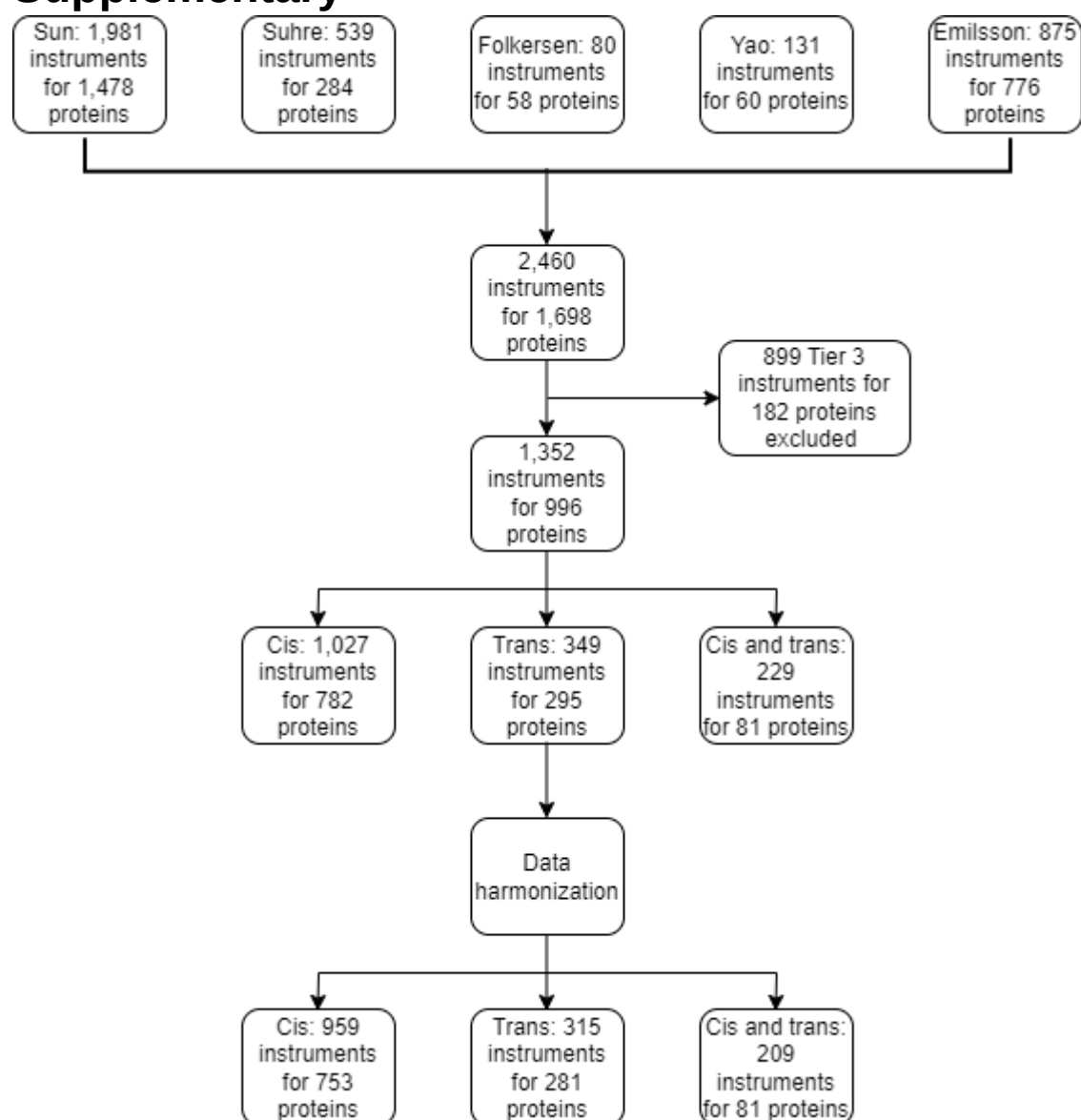
Supplementary figure 1 – a workflow of instruments (pQTL) used in our analysis
