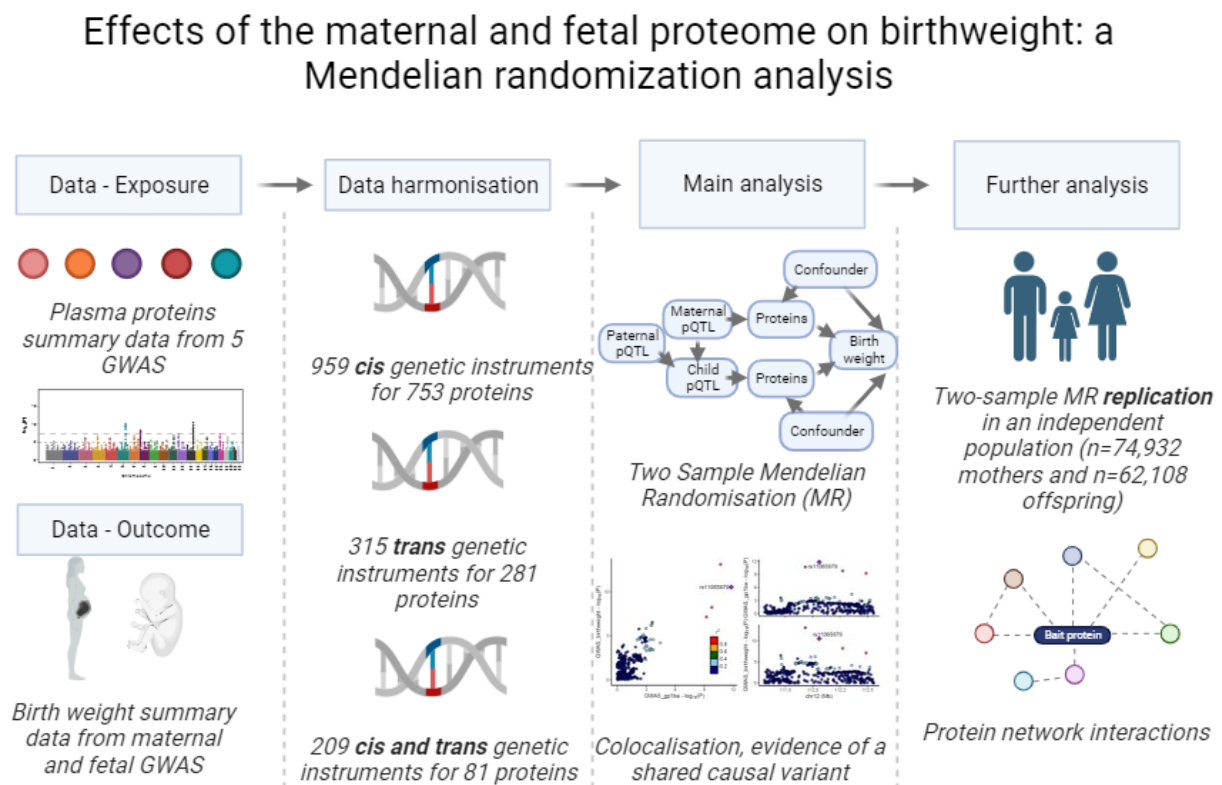
Figure 1 – Schematic representation of the analyses conducted in this paper. Abbreviations: GWAS, genome wide association studies; pQTL, protein quantitative trait loci
