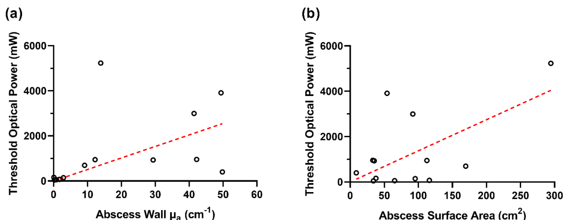
Figure 4. Relationship between optical power required to achieve a fluence rate of 4 mW/cm 2 in 95% of the abscess wall after treatment planning and (a) abscess wall \mu_a , or (b) abscess surface area, using flat cleaved fiber.
