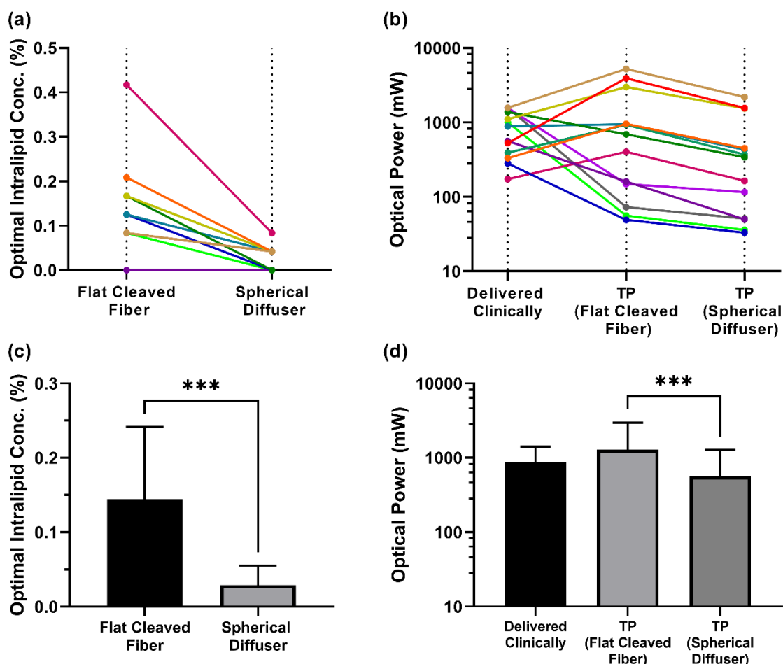
Figure 5. Comparison between flat-cleaved and spherical diffuser fibers for (a) optimal Intralipid concentration and (b) required optical power after treatment planning. Corresponding means and standard deviations are included for (c) optimal Intralipid concentration and (d) required optical power. *** p<0.001
