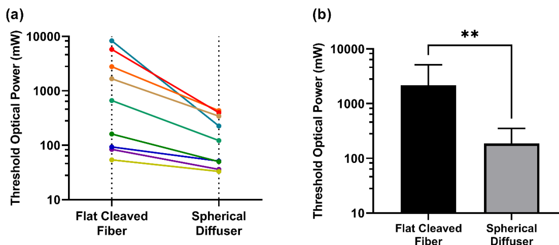
Figure 6. (a) Comparison of threshold optical power after treatment planning between flat cleaved fibers and spherical diffuser fibers for the case of 0% Intralipid concentration with (b) corresponding means and standard deviations across subjects. ** p<0.01
