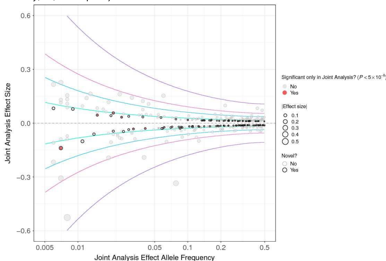
Figure 4. Plot of the relationship between minor allele frequency and estimated effect sizes for PSA GWAS significant variants. Each point represents one of the 447 independent genome-wide significant SNPs identified in our mJAM multi-ancestry GWAS joint meta-analysis. The SNP effect sizes are expressed in \ln(\text{PSA}) per minor allele. The curves indicate the hypothetical detectable SNP effect sizes for a given minor allele frequency, assuming statistical power of 80%, \alpha=5\text{e-}8 (genome-wide significant), and the sample size of each of our populations here (297,166 European ancestry, N=61,745 African ancestry, 6,967 Asian ancestry, 26,644 Hispanic).
