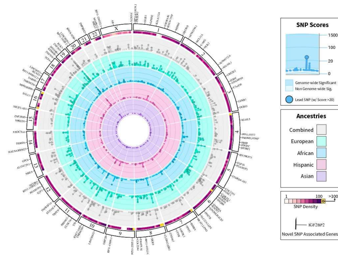
Figure 2. Circos plot showing PSA GWAS significant variants by chromosome from the discovery cohort. Concentric tracks are colored based on results from individual ancestries, with gray indicating results from the overall discovery meta-analysis. The top 100,000 GWAS SNPs (with the smallest p-values) per ancestry are shown as points; larger circled points indicate the 318 genome-wide significant variants ( p < 5e-8 ; 184 of which were novel) from the overall discovery analysis in all ancestries. SNP density in 10Mbp bins from the overall analysis is shown as a heatmap above the overall track. The outermost ring displays genes associated with novel discovery PSA SNPs.
