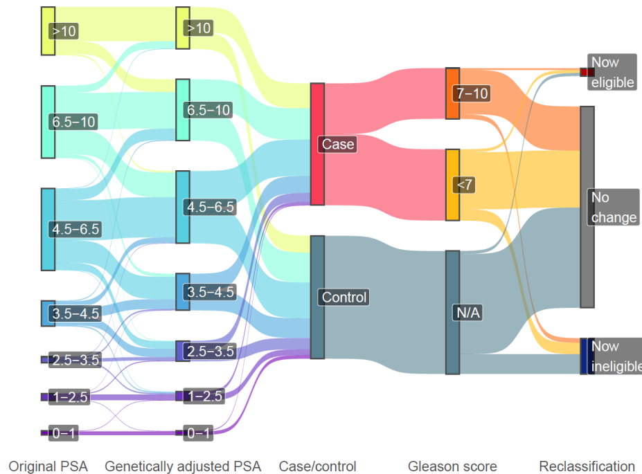
Figure 6. Biopsy reclassification with genetically-adjusted PSA. PSA levels were adjusted using the PRS-CSx estimate from the out-of-sample discovery cohort, assessed in GERA using age-specific cutoffs in (A) Europeans and (B) African Americans (see Methods ). GERA Latinos and East Asians are shown in Figure S3 .
