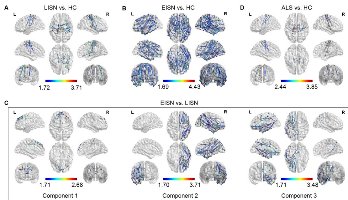
7 Figure 3. The impaired structural subnetworks in group comparisons based on the BNA
