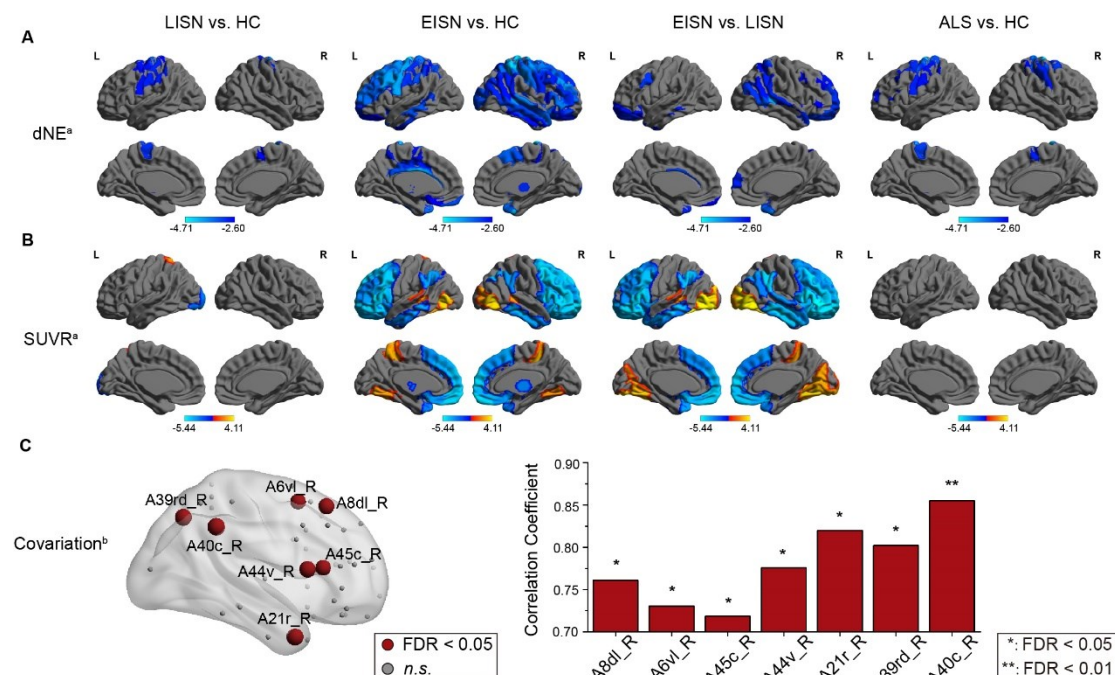
3 4 Figure 2. Distribution patterns of labels with decreases in dNE and changes in SUVR with the BNA
