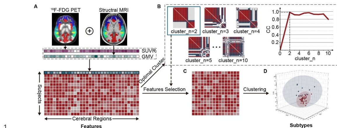
Figure 1. Cluster analysis procedure using ^{18}\text{F} -FDG PET/MR imaging
