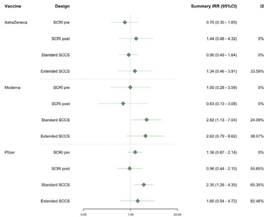
Figure 5: Meta-analysed adjusted association between the first dose of each vaccine and myocarditis, after adjustment for calendar time in 60-day increments
