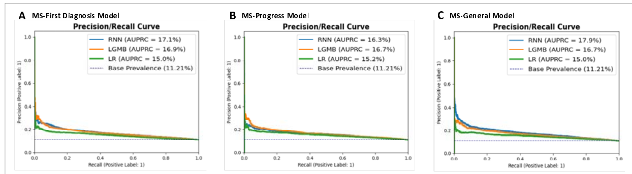
Figure 2: AUPRC curve of the MS-Diagnosis model (A), MS-Progress model (B), and MS-General model (C) tested on the MS-First Diagnosis test set
