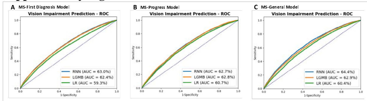
Figure 1: AUROC curve of the MS-Diagnosis model (A), MS-Progress model (B), and MS-General model (C) tested on the MS-First Diagnosis test set
