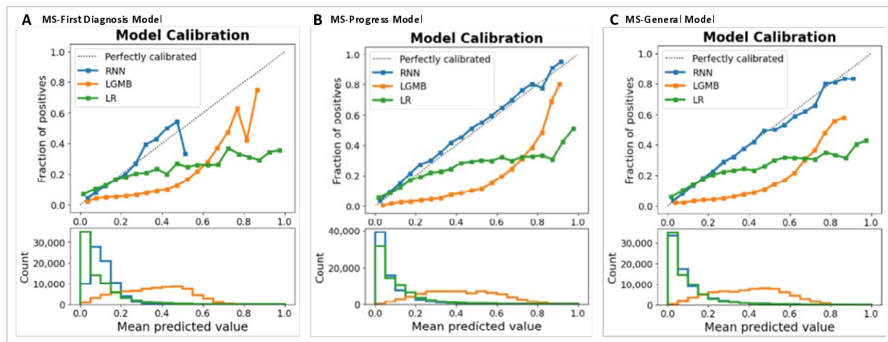
Figure 6: Calibration curve of the MS-Diagnosis model (A), MS-Progress model (B), and MS-General model (C) tested on the MS-Progress test set
