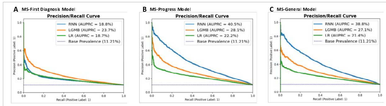
Figure 5: AUPRC curve of the MS-Diagnosis model (A), MS-Progress model (B), and MS-General model (C) tested on the MS-Progress test set
