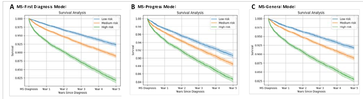
Figure 7: Kaplan-Meier curve of patients likely to have vision impairment within 5 years of the MS-Diagnosis model (A), MS-Progress model (B), and MS-General model (C) tested on the MS-First Diagnosis test set
