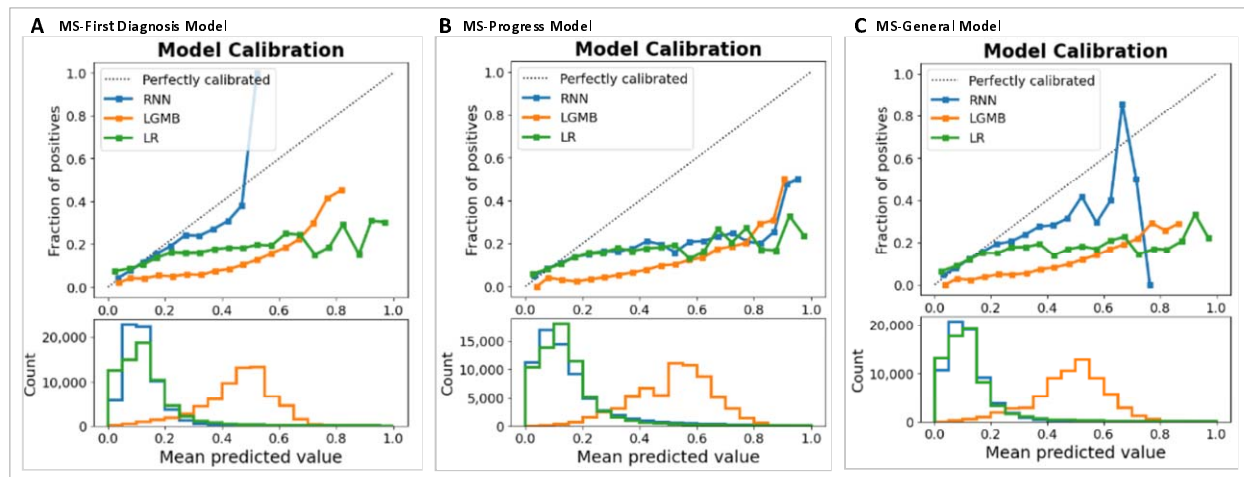
Figure 3: Calibration curve of the MS-Diagnosis model (A), MS-Progress model (B), and MS-General model (C) tested on the MS-First Diagnosis test set
