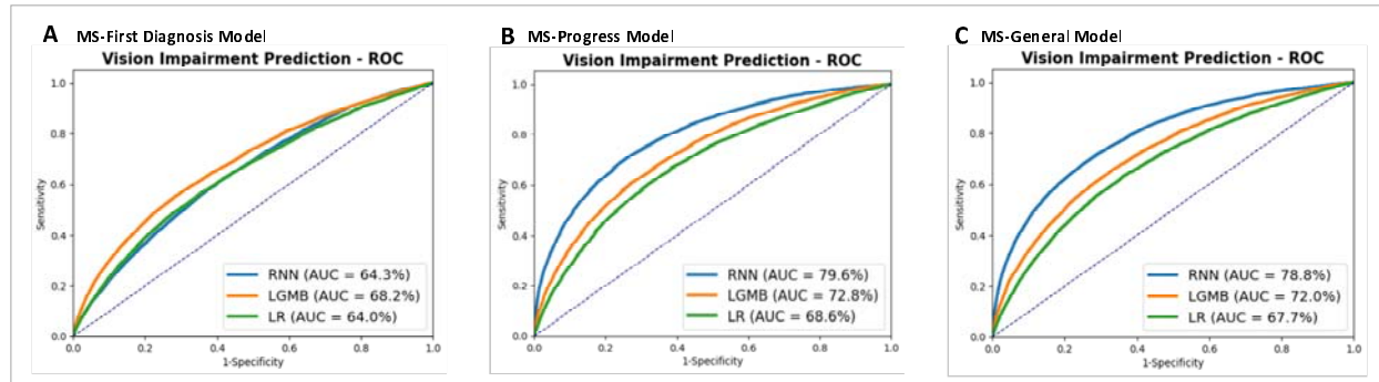
Figure 4: AUROC curve of the MS-Diagnosis model (A), MS-Progress model (B), and MS-General model (C) tested on the MS-Progress test set
