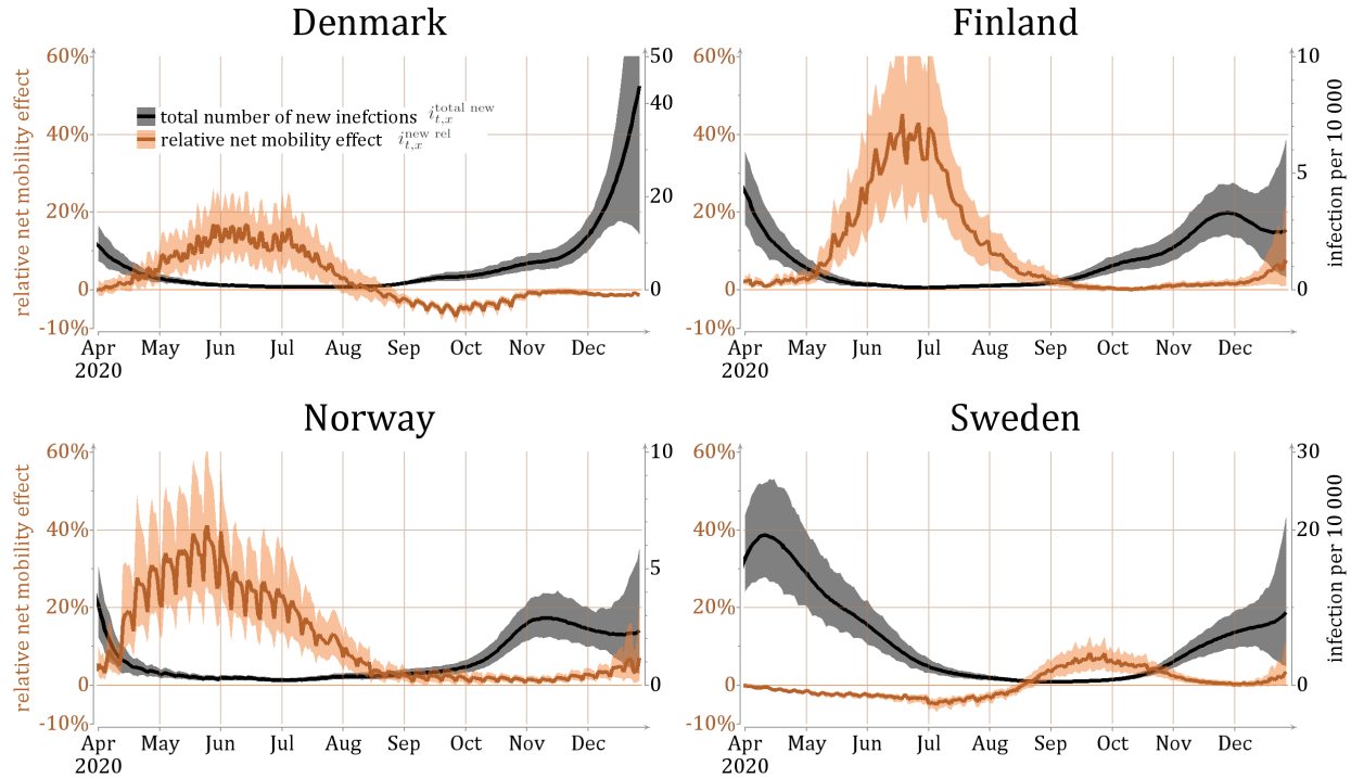
Figure 3: Black color: estimates of the total number of new infections i_{t,x}^{total new} of equation (12) per day per 10,000 individuals (lines show posterior mean and colored areas show 90% posterior intervals). Orange: estimates of the relative net mobility effect of equation (15) i_{t,x}^{new rel} , defined by dividing the net mobility effect (cf. equation (14)) by the total number of new infections (lines show posterior mean and colored areas show 90% posterior intervals).
