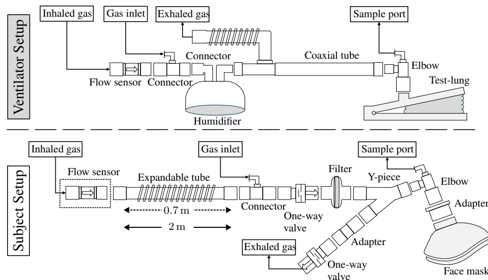
Figure 2. A schematic representation of the respiratory circuits employed in mechanical ventilation of a test-lung (Ventilator Setup) and spontaneous breathing among healthy subjects (Subject Setup). In the Ventilator Setup, the respiratory circuit encompasses a flow sensor affixed to the outlet of the ventilator (not depicted), followed by a connector equipped with a luer-port to facilitate the introduction of additional CO 2 . To ensure the homogeneity of the gas mixture, an empty humidifier was incorporated to enable air mixing. A coaxial tube connected to the humidifier and to the ventilator's inlet, with the distal end attached to the test-lung via an elbow featuring a sampling port. In the Subject Setup, the configuration of the respiratory circuit differed slightly for the Additional CO 2 and Reservoir CO 2 Systems. In the Reservoir CO 2 configuration, the deployment of a flow sensor was omitted, and the extendable tube was elongated from its minimal length of 0.7 m, as utilized in the Additional CO 2 configuration, to a length of 2 m, serving as a reservoir for the added gas. The expandable tube was affixed to the gas inlet connector, followed by one-way valves and a Y-connector separating the inhalation and exhalation part of the circuit. A filter prevented particles reaching the subjects who breathing in the circuit through a face mask which was fitted to the head with the help of an adjustable harness (not shown).
