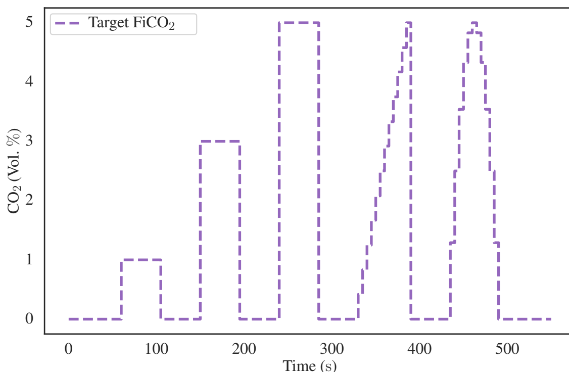
Figure 3. The CO 2 target function employed for the assessment of the precision of the proposed Additional CO 2 method. The target function comprises three 45 s box-stimulus intervals, each at distinct CO 2 concentrations of 1 %, 3 % and 5 %. These stimuli were subsequently followed by a 60 s ramp and half-sinusoidal waveform, both characterized by a peak concentration of 5 % CO 2 . A 45 s baseline was inserted between each stimulus and an initial and final baseline of 60 s duration was also included.
