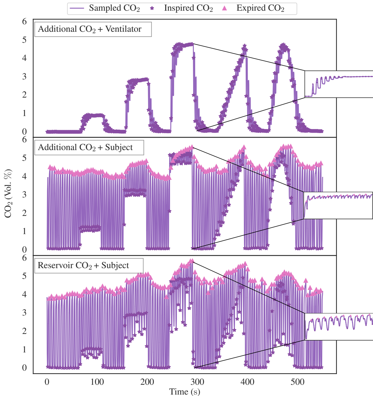
Figure 4. Illustrative data pertaining to FiCO 2 target accuracy assessment, delineating the three distinct experimental configurations: the Additional CO 2 System + Ventilator Setup (depicted in the top graph), the Additional CO 2 System + Subject Setup (displayed in the middle graph), and the Reservoir CO 2 System + Subject Setup (depicted in the bottom graph). All three instances use the identical target function as showcased in figure 3. Upon closer examination within the magnified window, we see the dynamic fluctuations in CO 2 concentration throughout the 5 % box-stimulus. It becomes evident that the rise time of CO 2 in the Ventilator Setup exhibits a substantially slower response in comparison to the other two configurations. Furthermore, the Reservoir CO 2 System manifests a markedly greater degree of variability in inspired CO 2 levels when compared with the Additional CO 2 System.
