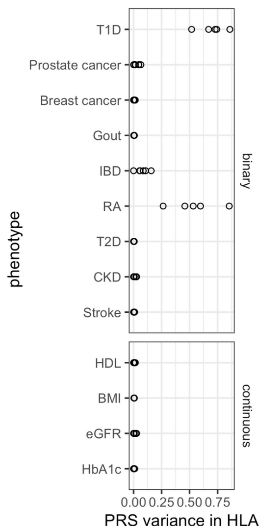
1150 Supplementary Figure 16: PGS variance originating in the HLA region for the scores used to estimate \tau_{\text{biobank}} and \tau_{\text{method}} in EUR ancestry target data
