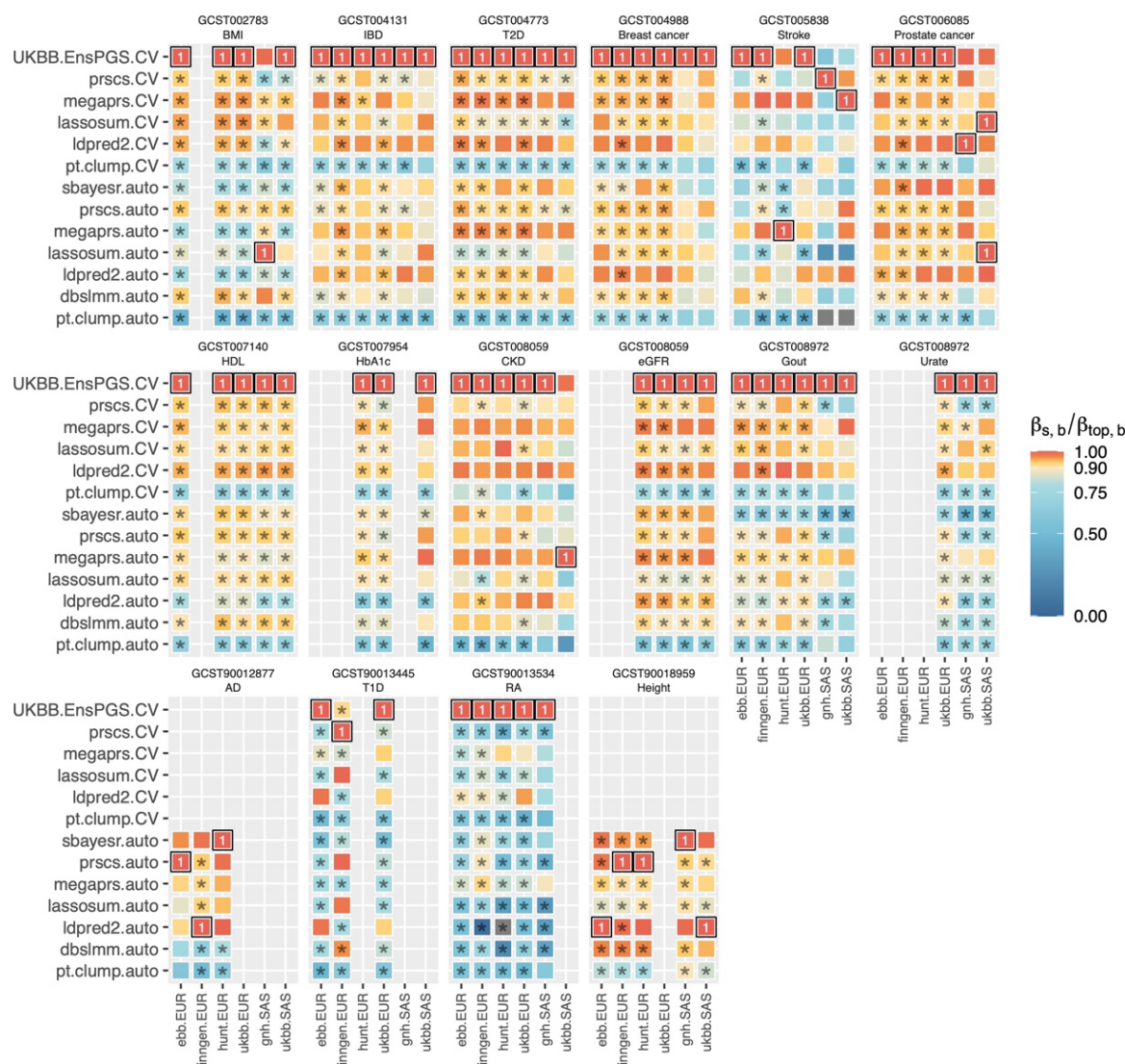
Supplementary Figure 9: Relative PGS effect sizes ( \beta_{s,b}/\beta_{top,b} ) across 16 traits within biobanks and ancestries
