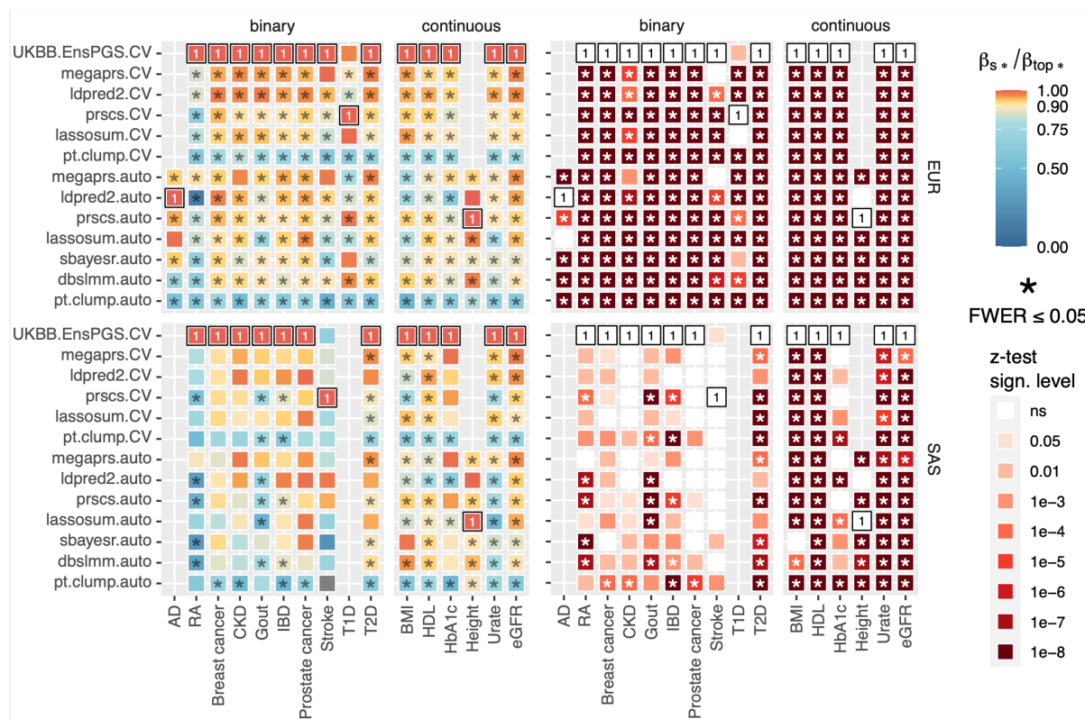
Supplementary Figure 6: Relative meta-analyzed PGS effect sizes across 16 traits
