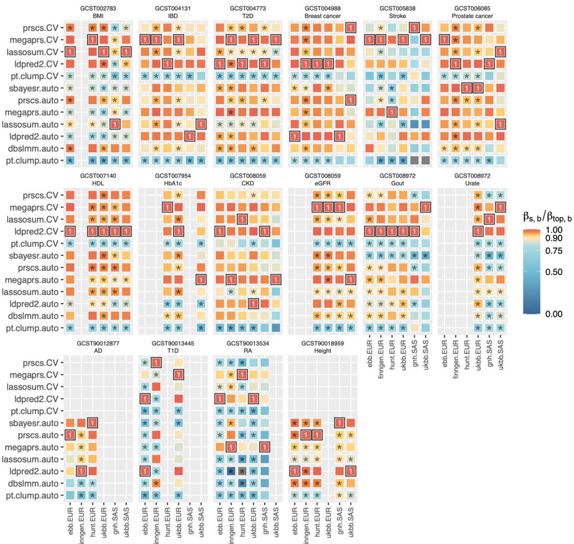
Supplementary Figure 10: Relative PGS effect sizes ( \beta_{s,b}/\beta_{top,b} ) across 16 traits within biobanks and ancestries excluding the ensemble PGS
