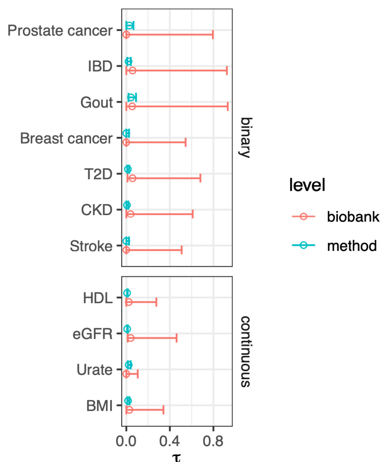
Supplementary Figure 14: \tau_{\text{biobank}} and \tau_{\text{method}} estimated in SAS ancestry target data
