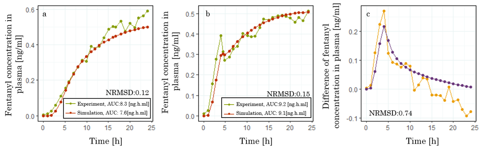
Figure 7- Validation of prediction of digital twin on the impact of heat on fentanyl concentration in plasma
