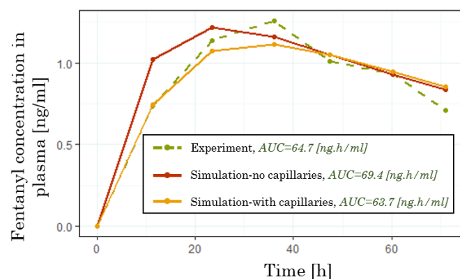
Figure 5- Fentanyl concentration in the plasma during 72 hours of applying one fentanyl patch with a nominal flux of 50 \mu\text{g}/\text{h} . (The green curve is based on results from the Marier et al. study (Marier et al. 2006), and the red curve is based on results from the Bahrami et al. study (Bahrami, Rossi, and Defraeye 2022)).
