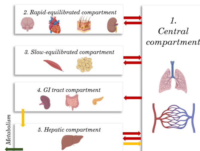
Figure 3- The compartments involved in the pharmacokinetics model. (Created with BioRender.com)
