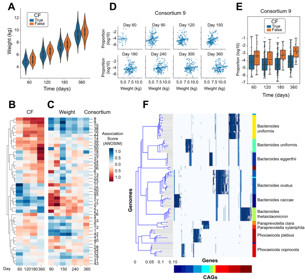
Figure 4. Association of specific microbial consortia with infant CF status and weight.
