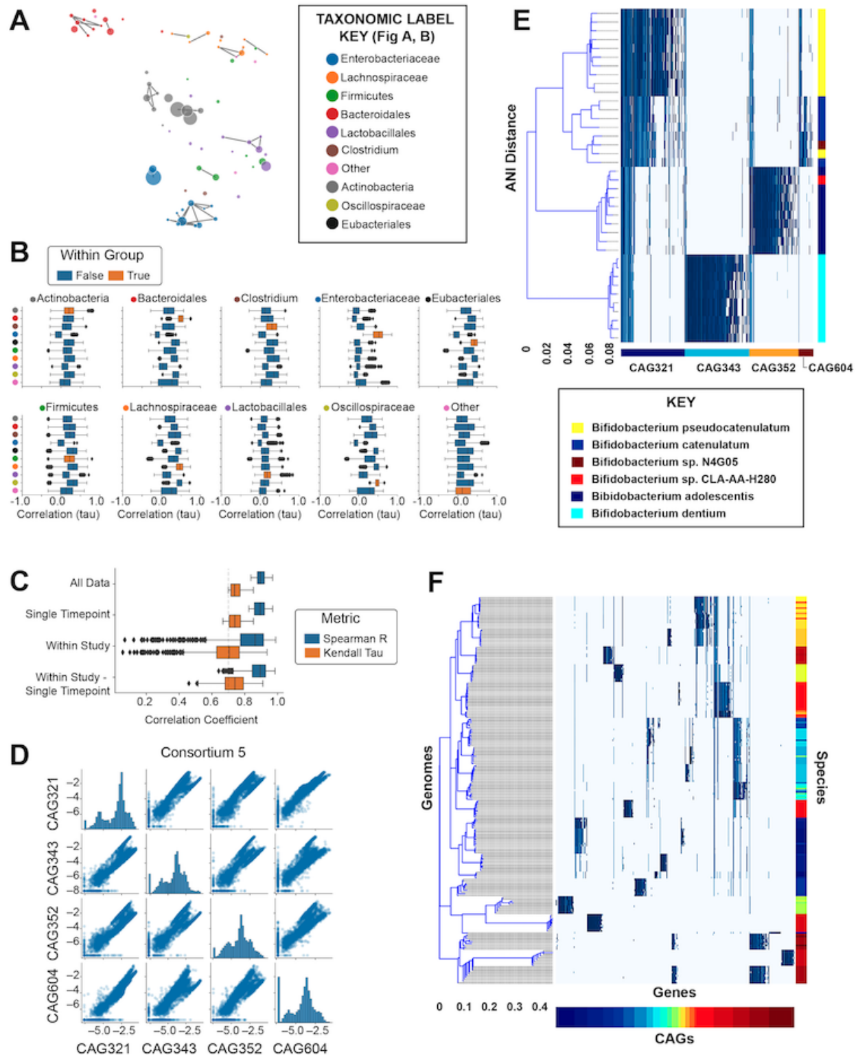
Figure 2. Groups of microbial genomospecies are reproducibly observed at correlated abundances across studies.
