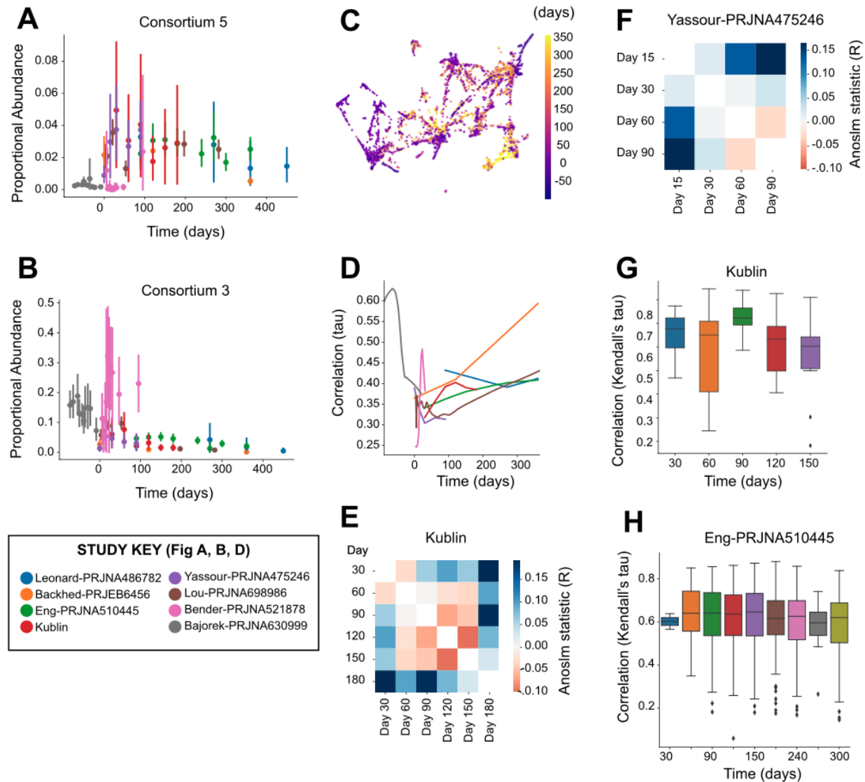
Figure 3. Rapid changes in relative abundance of microbial consortia during early human life.
