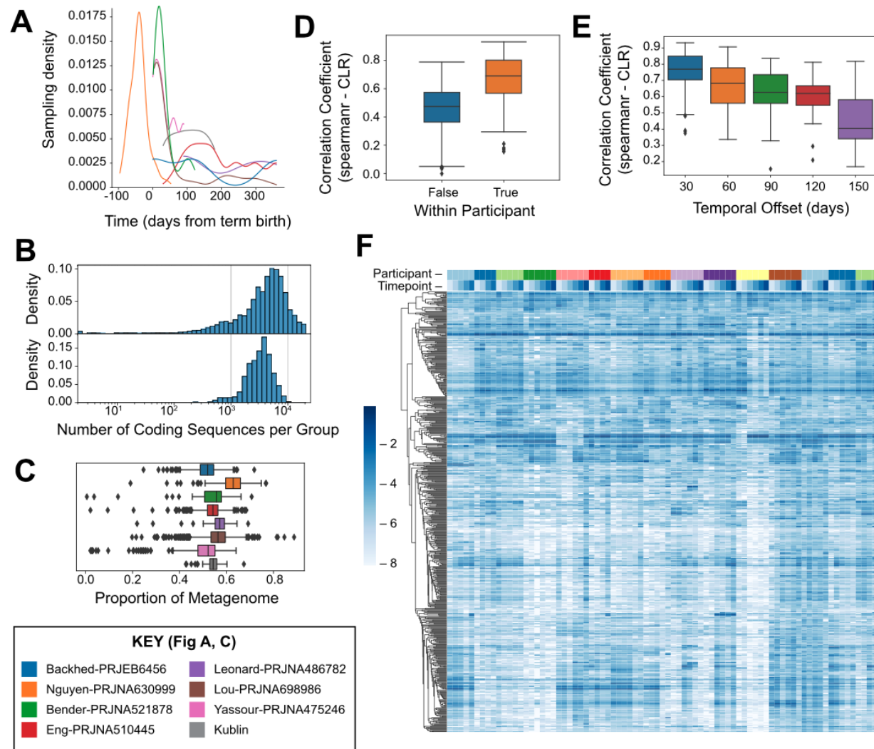
Figure 1. Quantification of 592 microbial genomespecies from 0-6 months across 8 studies.
