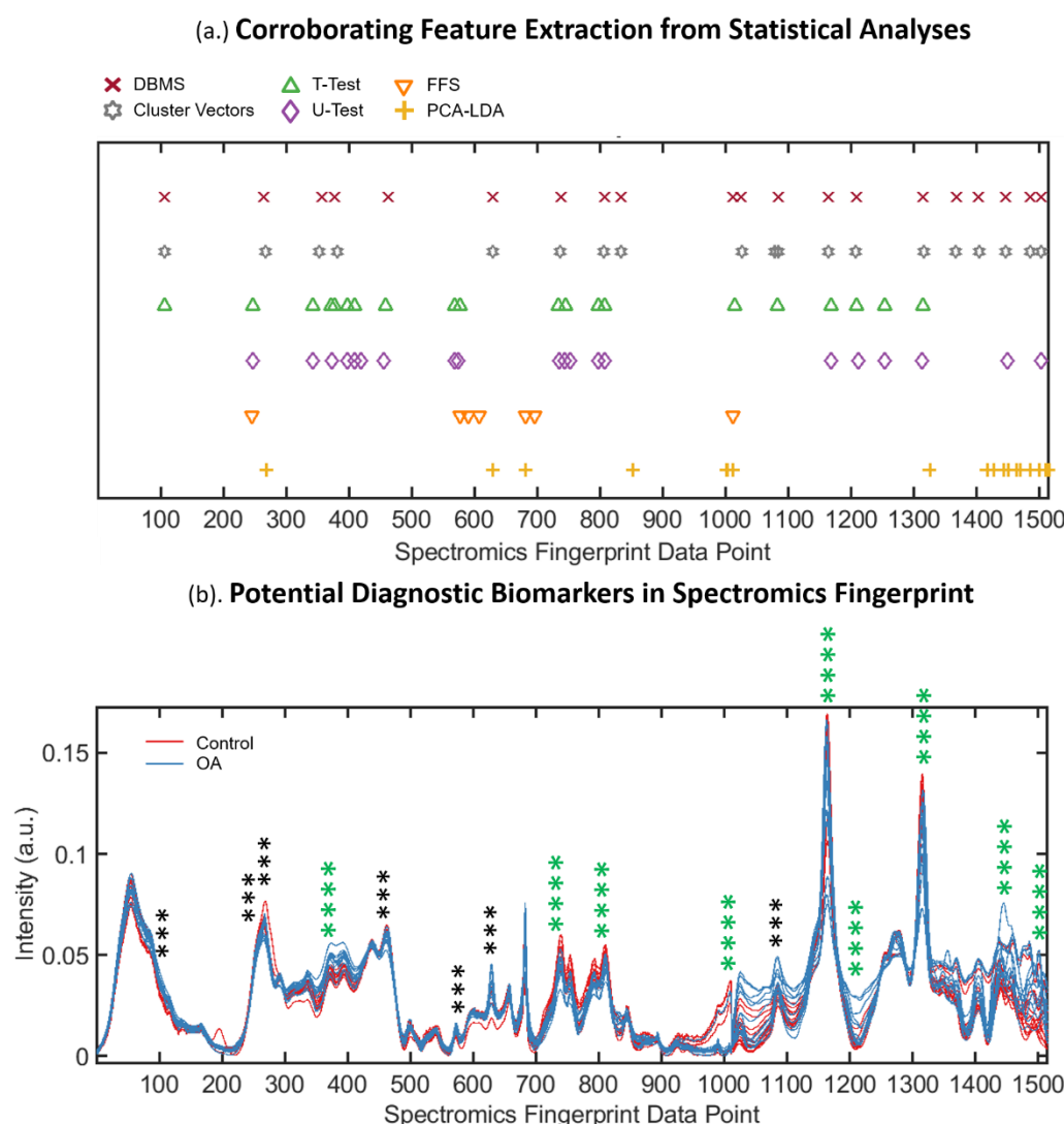
Fig. 4: Candidate spectral biomarkers identified by corroboration between the highest scoring features extracted by separate statistical tests. (a.) Highest scoring features presented for Difference Between Mean Spectra, Cluster Vector Analysis, Student's T-test, Mann-Whitney U-Test, Feature Forward Selection, and weightings for PCA-LDA. (b.) Corroborating the statistical tests sees certain spectral regions in agreement, displayed as regions scoring four or three hits.
