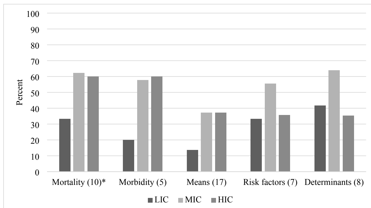
Figure 2. Percent of reported SDG health-related indicators in EMR Voluntary National Reports, by income levels
