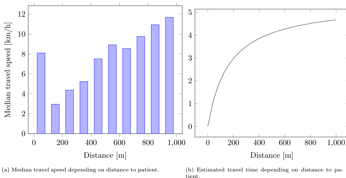
Figure 3: Distance-dependent travel times estimated based on historical data.
