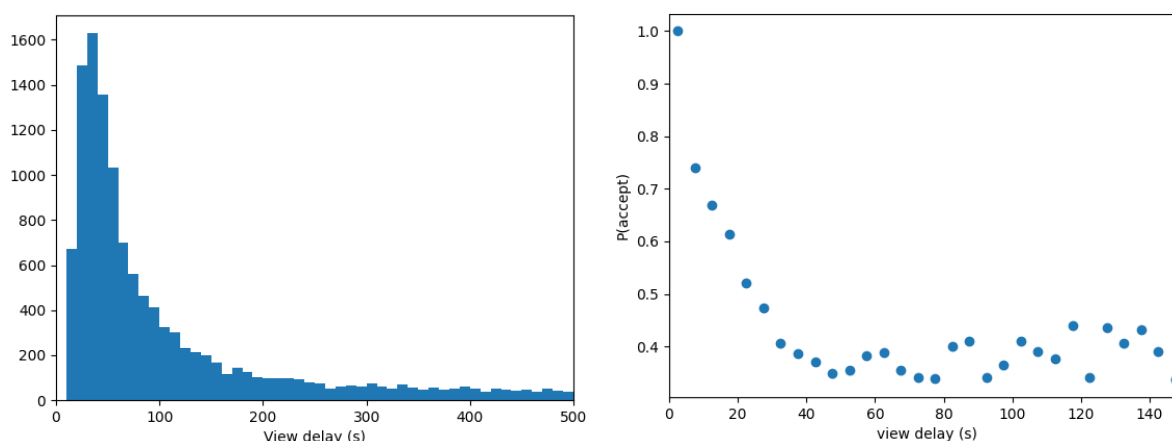
Figure 2: Historical view delays and acceptance probabilities as observed on GoodSAM in New Zealand.
