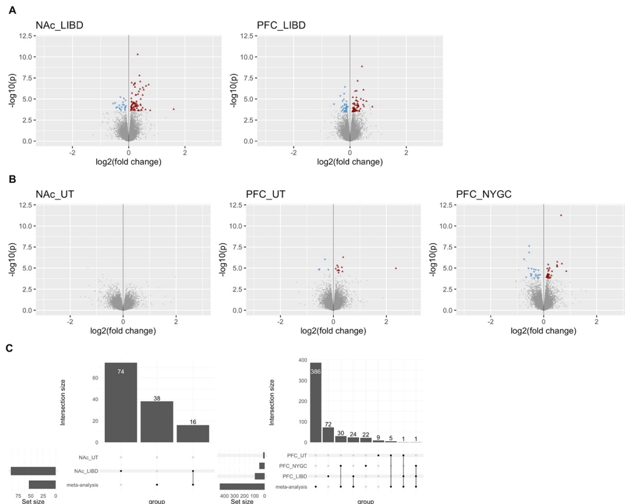
Figure 2. (A) Volcano plots of the differentially expressed genes (FDR < 0.05) by AUD status in the LIBD datasets. Blue triangles represent significant downregulated genes and red triangles represent significantly upregulated genes. Genes not significantly differentially expressed are colored grey. (B) Volcano plots of the differentially expressed genes (FDR < 0.05) by AUD status in the NSW-TRC datasets. Blue triangles represent significant downregulated genes and red triangles represent significantly upregulated genes. Genes not significantly differentially expressed are colored grey. (C) Upset plots displaying the gene overlap count between the individual datasets DEGs and meta-analysis DEGs by brain region.
