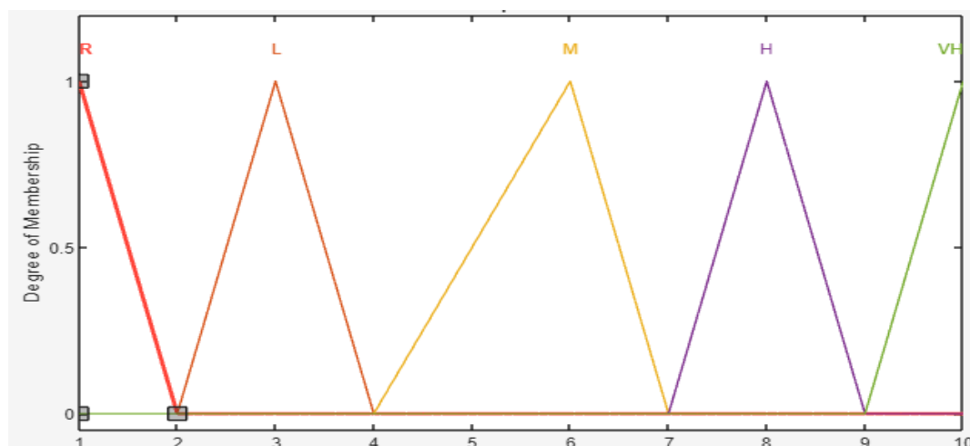
Figure 4: Membership function plot for Occurrence. R: Remote, L: Low, M: Moderate, H: High, VH; Very High.
