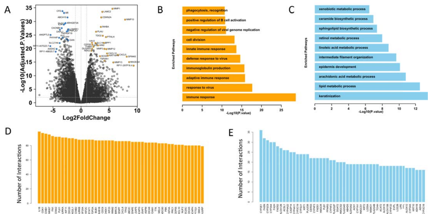
Figure 2. RNA-seq analysis.
