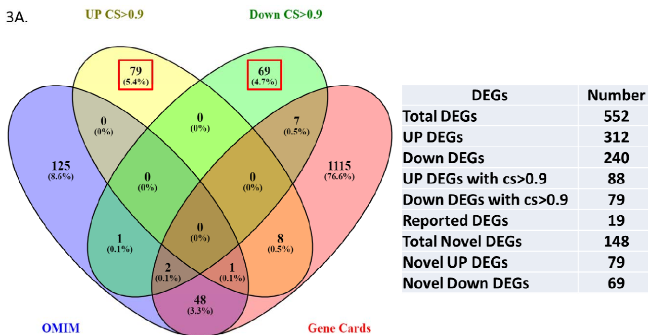
Figure 3: Venn diagram of the differentially expressed genes (DEGs).
