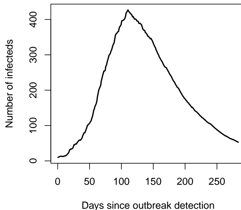
Figure 13: Expected number of infecteds over time.
