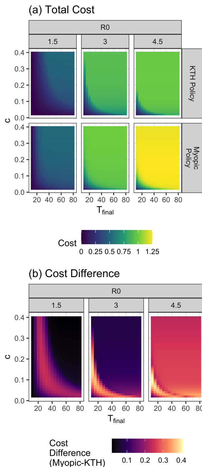
Figure 4. (a) Total costs for the full optimization and myopic solutions. (b) Difference in total costs for solutions resulting from the myopic solutions and full optimization. Values of T_{\text{final}} , c and R_0 are shown in the figure. i_0 = 0.0001 . A cost of 1 is equivalent to the cost of the entire population becoming infected.
