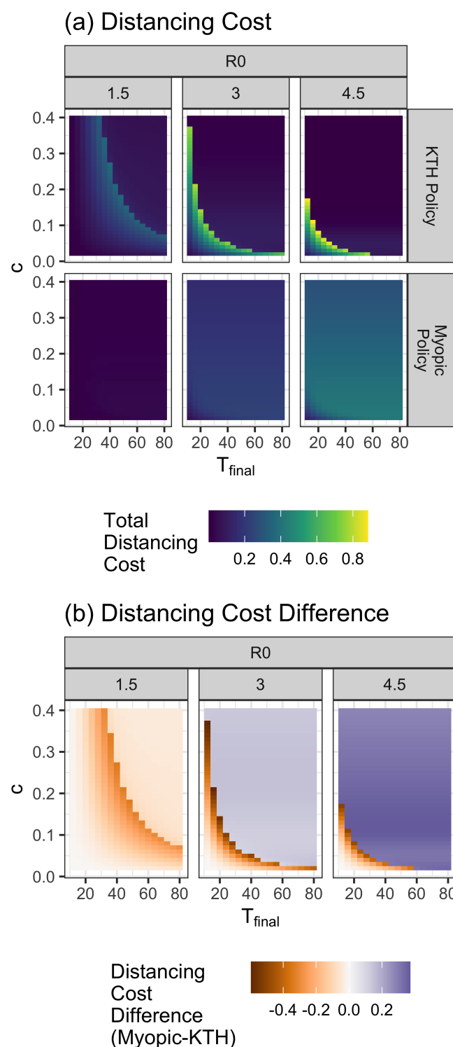
Figure 3. (a) This figure shows the distancing cost for both the KTH and myopic policies. (b) The differences between the myopic distancing cost and the KTH distancing cost are shown. Values of T_{\text{final}} , c and R_0 are shown in the figure. i_0 = 0.0001 . A cost of 1 is equivalent to the cost of the entire population becoming infected.
