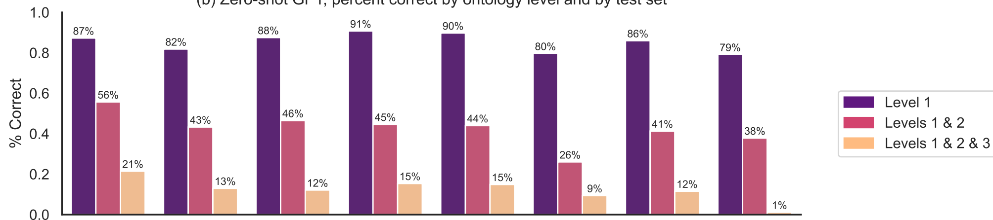
(b) Zero-shot GPT, percent correct by ontology level and by test set
