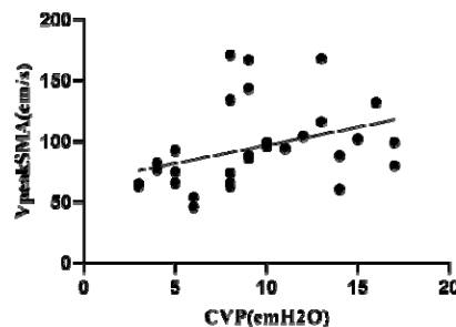
Fig 9. Scatter diagram of VpeakSMA and CVP
