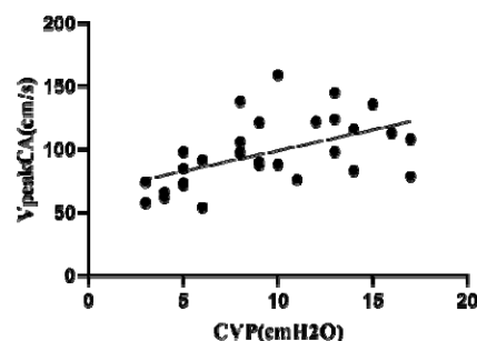
Fig 5. Scatter diagram of VpeakCA and CVP
