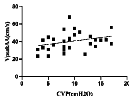
Fig 1. Scatter diagram of VpeakAA and CVP
