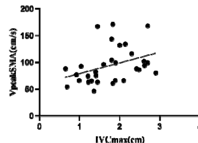
Fig 10. Scatter diagram of VpeakSMA and IVCmax
