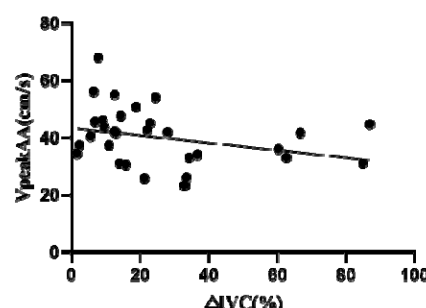
Fig 3. Scatter diagram of VpeakAA and \Delta IVC
