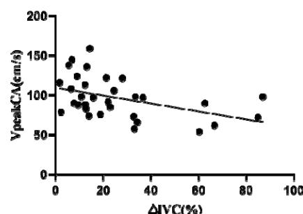
Fig 7. Scatter diagram of VpeakCA and \Delta IVC
