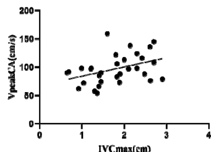
Fig 6. Scatter diagram of VpeakCA and IVCmax
