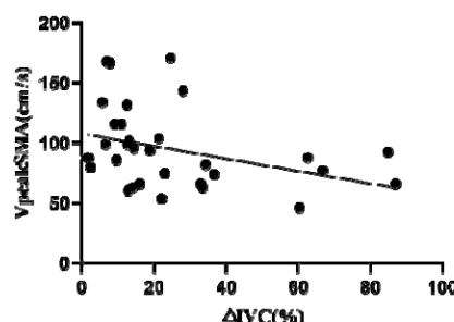
Fig 11. Scatter diagram of VpeakSMA and ΔIVC
