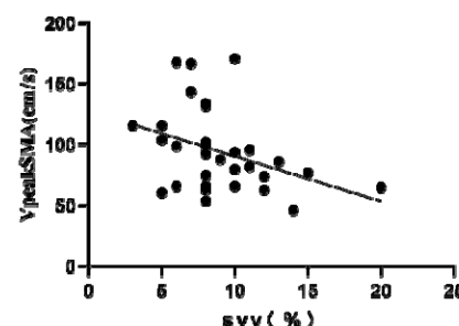
Fig 12. Scatter diagram of VpeakSMA and SVV
