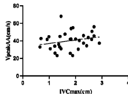
Fig 2. Scatter diagram of VpeakAA and IVCmax
