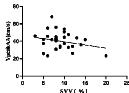
Fig 4. Scatter diagram of VpeakAA and SVV
