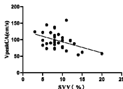
Fig 8. Scatter diagram of VpeakCA and SVV
