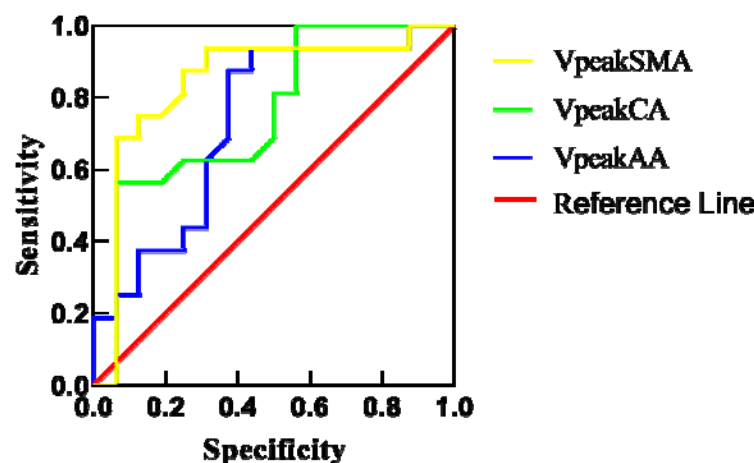
Fig 13.ROC curve of VpeakAA, VpeakCA and VpeakSMA for evaluating capacity status
