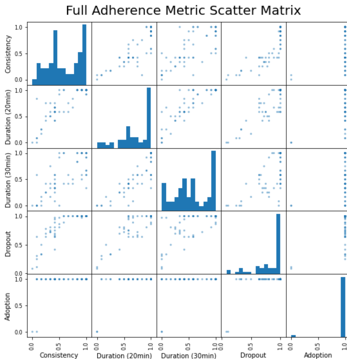
Figure 5: The relationship between adherence metrics. Each participant is assigned a normalised score for each metric. The diagonals show the score distribution for each metric, and the off-diagonals show the pairwise relationship.
