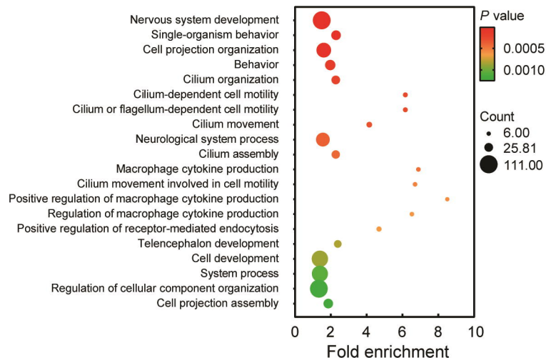
A Enriched genes
