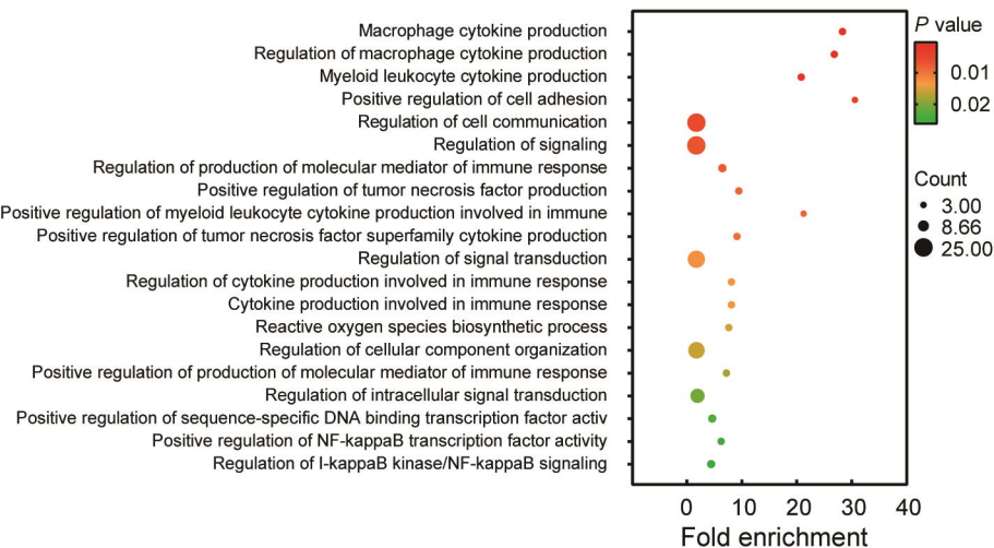
C Early-onset-specific genes
