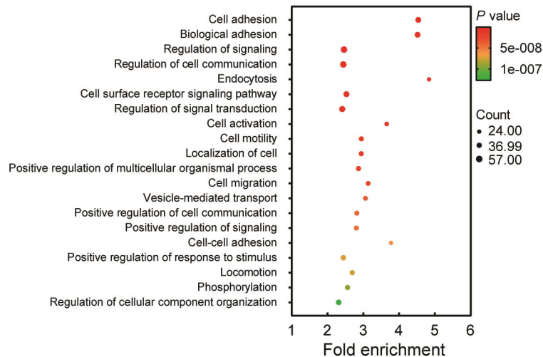
B Immune-related genes
