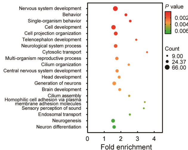
D Regular- and late-onset-specific genes
