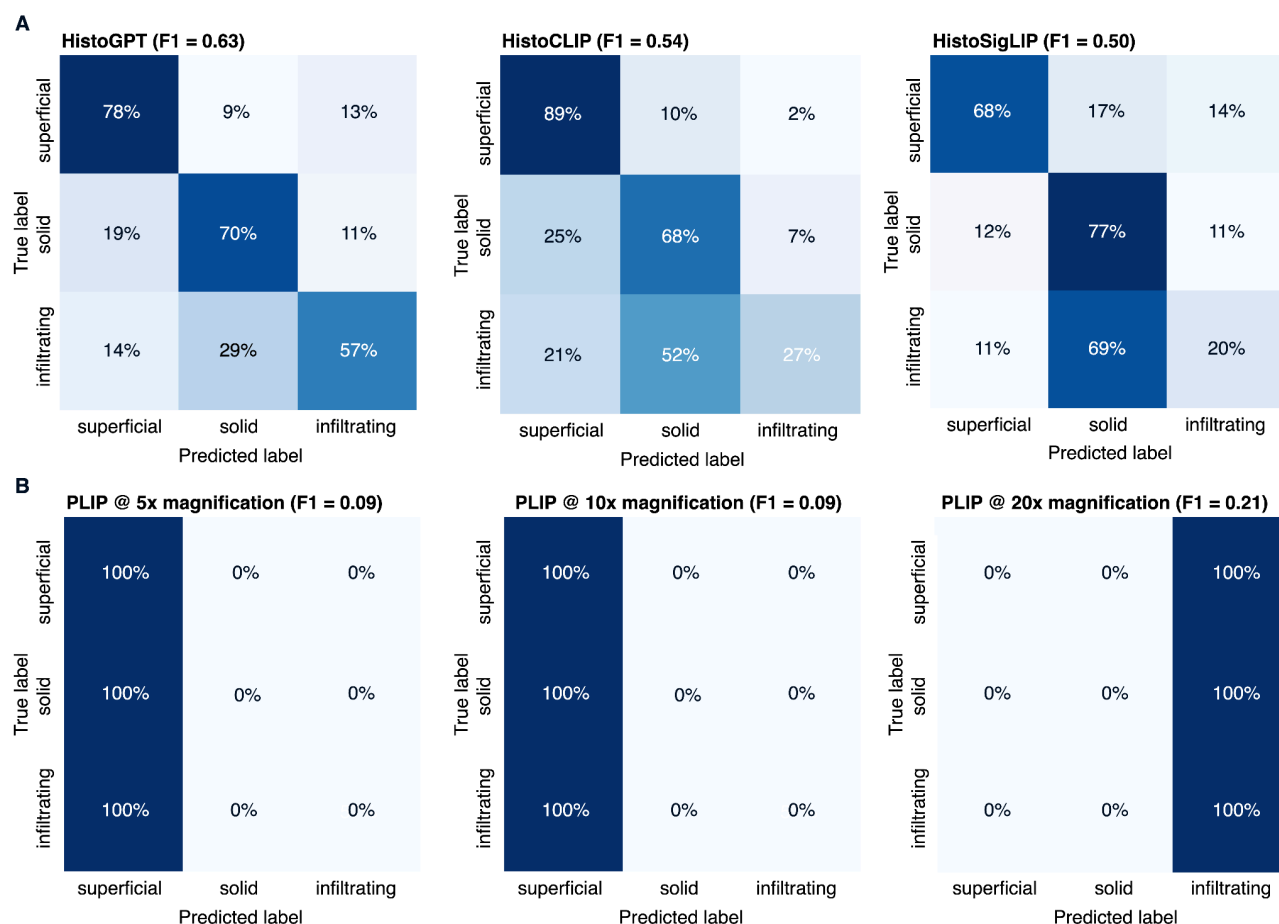
Supplementary Figure 5. Zero-shot tumor subtype prediction results summarized as a confusion matrix for HistoGPT-M, HistoCLIP, HistoSigLIP, and PLIP.
