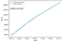
Florida:Deaths Prediction
