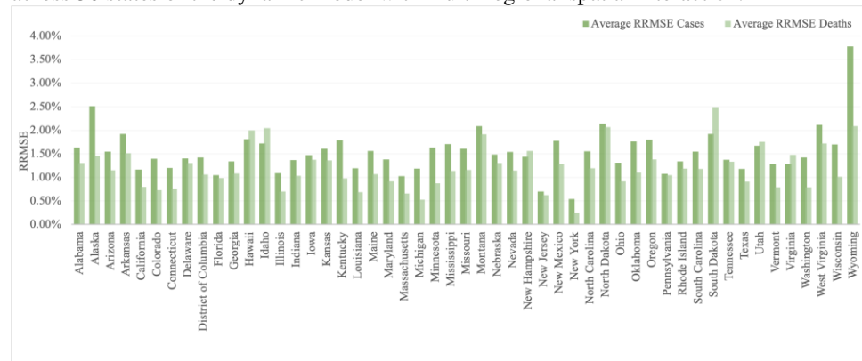
Fig. 3. Average RRMSE for Cases and Deaths over 7 Months Among 50 States ( \alpha=1, \gamma=2 )
