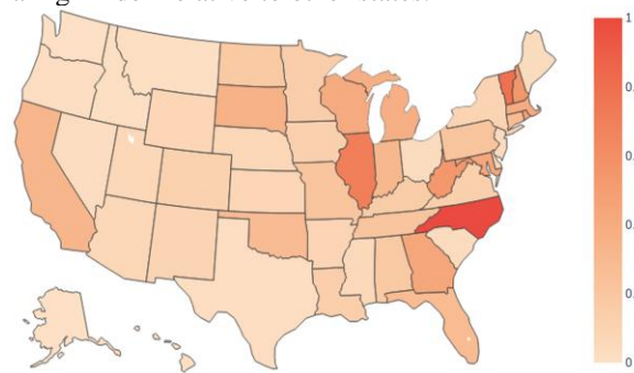
Fig. 8. Transmission Import Index Heat Map in the US from 03/20/2020 to 04/15/2020 ( \alpha = 1, \gamma = 2 )
