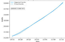
New Jersey:Deaths Prediction
