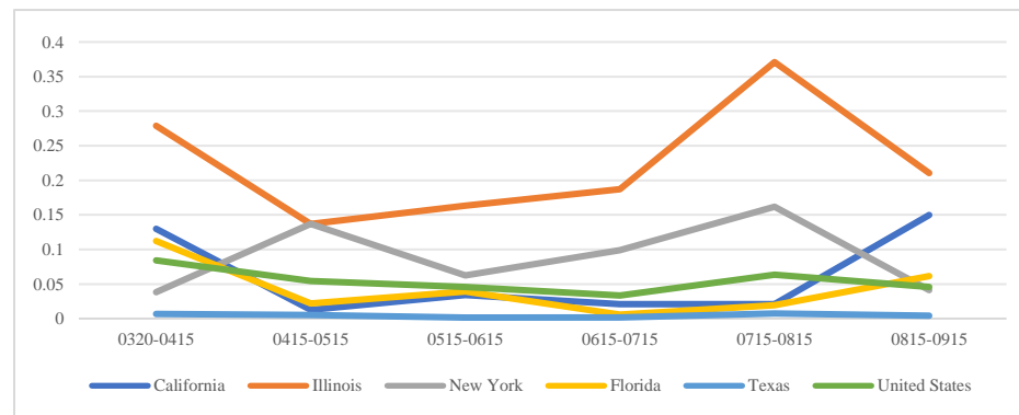
Fig. 6. Transmission Import Index for Six States in the US from 03/20/2020 to 09/15/2020 ( \alpha=1 , \gamma=2 )
