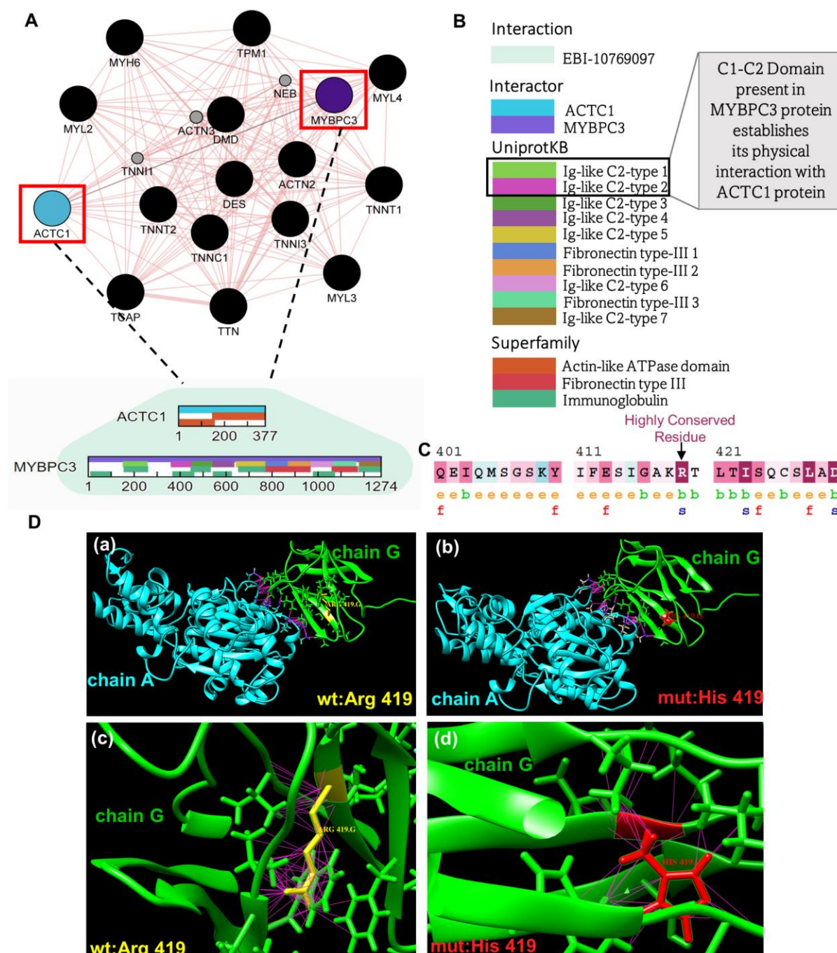
Fig 4: Analysis of the MYBPC3-ACTC1 interaction in the PPIN. A. MCL-cluster1 from the PPIN (Shown in S1_Fig and S2_Fig) is illustrated with nodes representing proteins ('black' filled circles) and edges indicating direct physical interactions between them. Notably, the proteins MYBPC3 and ACTC1 are highlighted in 'purple' and 'blue', respectively, with their interaction denoted by a 'green' edge. B. Domain architecture in the interaction between MYBPC3 and ACTC1. C. Evolutionary conservation analysis of MYBPC3 protein showing conserved residues. D. (a, b) MYBPC3:chainG and ACTC1:chainA protein complex showing intermolecular contacts ('pink') within ACTC1:chainA ('cyan') and MYBPC3:chainG ('green') with wild-type residue 'Arg' (shown in 'yellow') and mutated residue 'His' (shown in 'red') at position 419 of MYBPC3:chainG. (c, d) Number of contacts ('pink') for wild-type residue 'Arg419' and mutated residue 'His419'.
