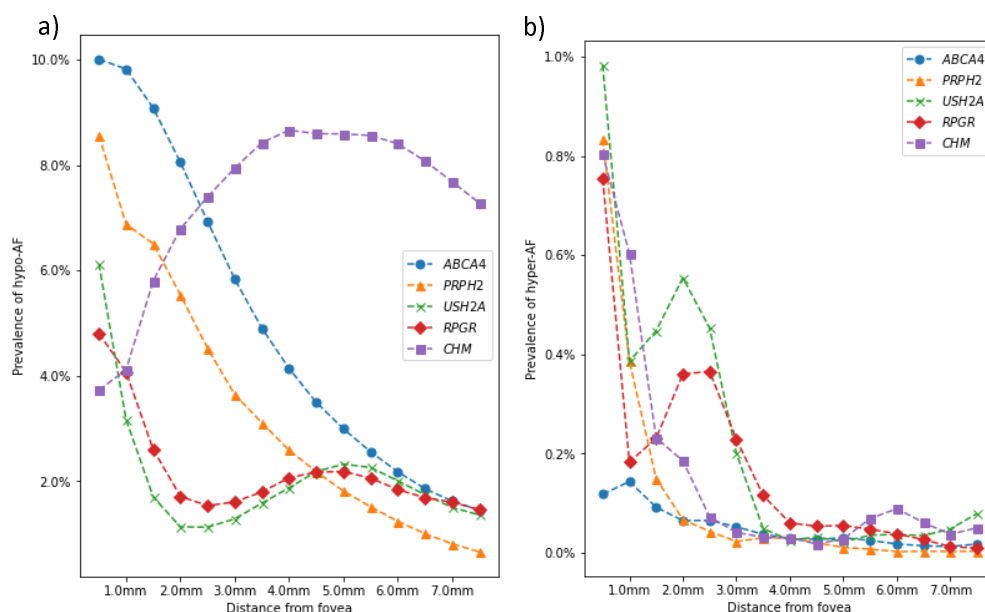
Figure 3: Autofluorescence (AF) as a proportion of total altered AF area in the image compared with distance from fovea for patients with variants in ABCA4 , PRPH2 , USH2A , RPGR , and CHM for a) hypo-AF and b) hyper-AF.
