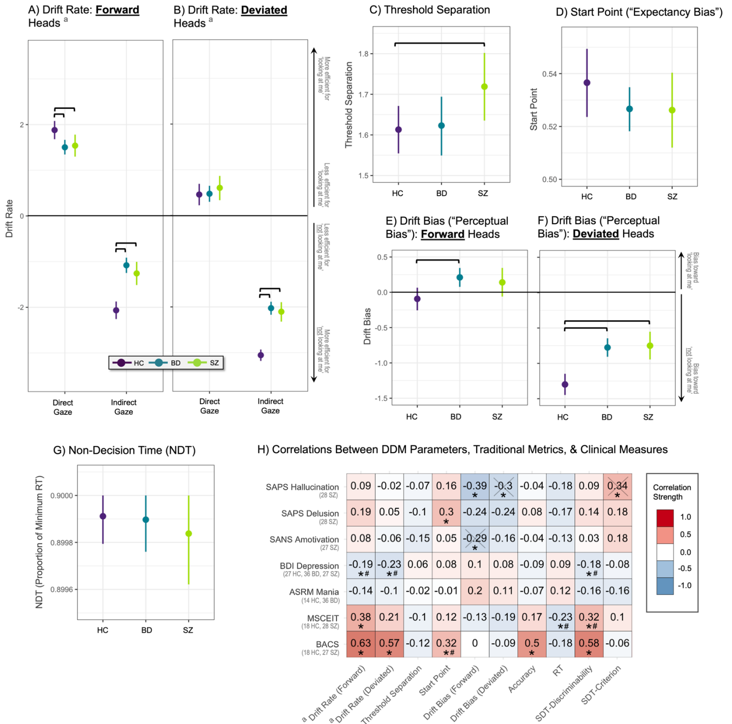
Figure 3. A-G) Group differences in DDM parameters. H) Zero-order correlations between DDM parameters, traditional performance metrics, general/social cognition, and SZ symptoms. Panels A-G: Points and error bars represent the mean and 90% highest density interval (HDI) of group posteriors, respectively. Horizontal black brackets indicate credible differences that do not contain zero. Panel G: NDT is a proportion of the minimum RT. Panel H: Values shown are mean posterior estimates of correlation coefficients (equivalent to Pearson R). The number of participants with valid data for each clinical metric is noted in the row labels. * = Credible zero-order association (i.e., 90% HDI does not contain zero); X = zero-order associations that were credible in the full sample, but were not robust to removal of influential cases; # = zero-order associations that were credible in the full sample, but were not also credible within SZ and/or BD patient groups; BACS = brief assessment of cognition in
