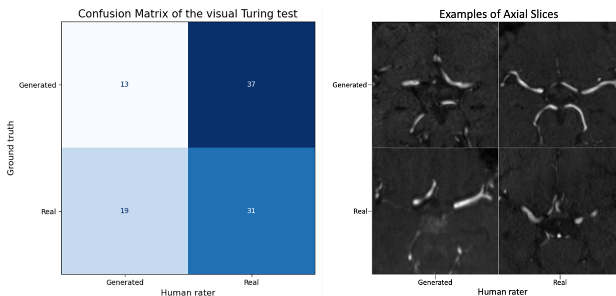
Figure 6. Visual Turing test results. The confusion matrix of the visual Turingon is shown (left). One example axial slice from each category (false positive, true positive, true negative, false negative) is shown (right).
